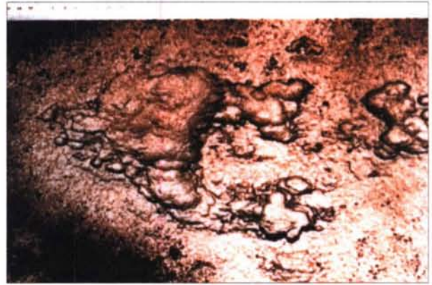
FIGURE 7. Close-up of sand-blasted surface showing MIC pattern. 52 Reproduced with permission from The Gas Technology Institute.
