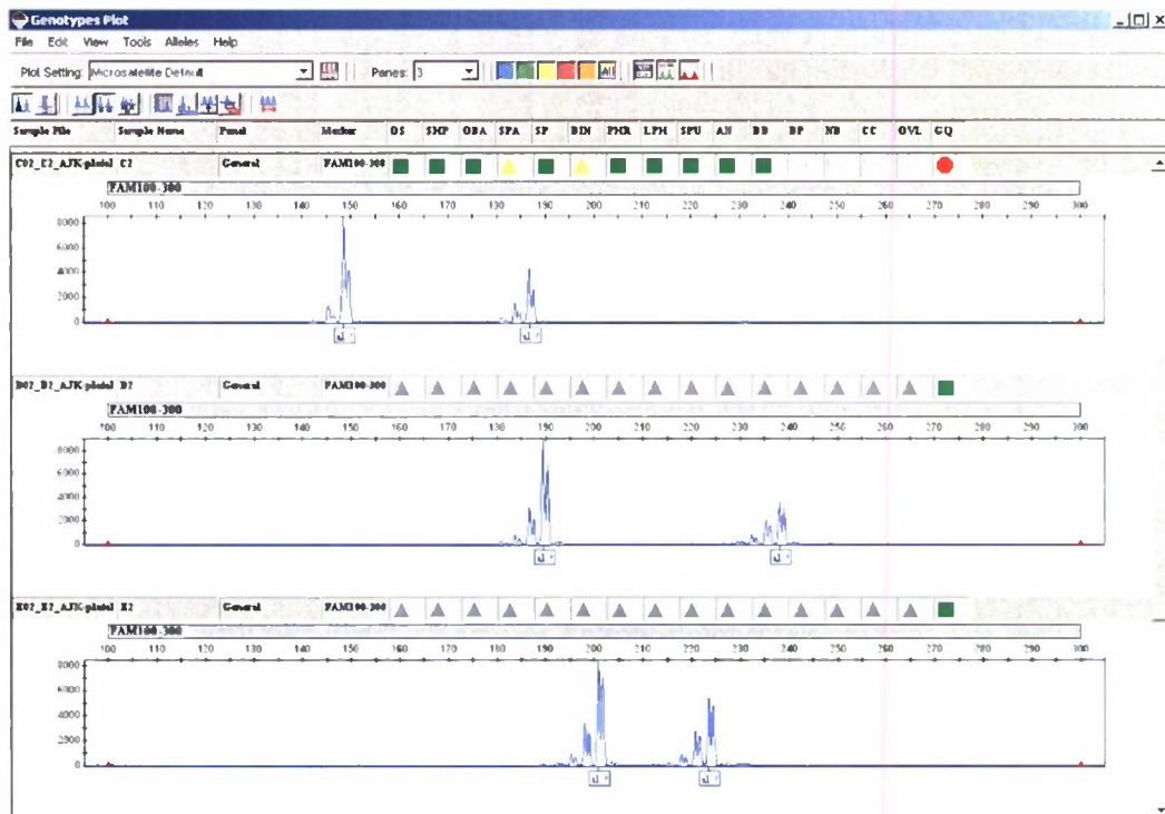
Figure B.4 Microsatellite electropherogram profile for locus Rpa10CA02.
