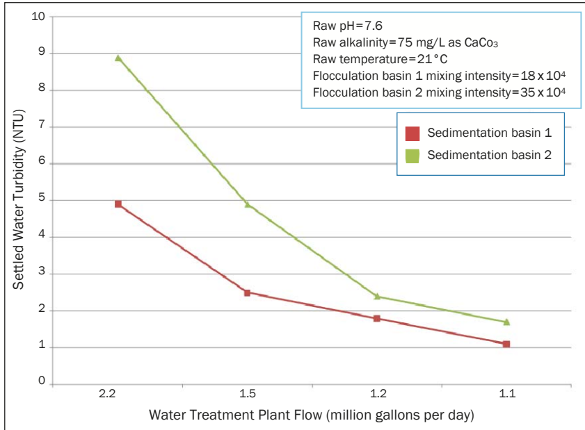
Figure 8. Jar test simulating basin 1 and basin 2 turbidity removal performance.
