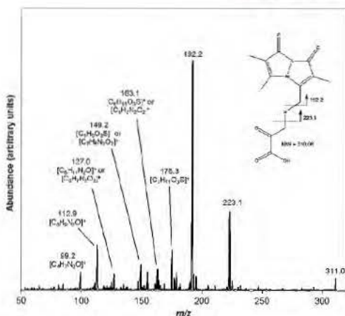
Fig. 3. The mass spectrum of the 3-MPB complex with tentative identification of the abundant ions. The 311 m/z ion corresponds to [M-H].
