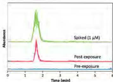
Fig. 3. Chromatograms of \alpha -K g CN spiked swine plasma (upper trace) and the plasma of cyanide-exposed swine, pre-exposure (lower trace), and post-exposure (middle trace). The chromatograms represent the signal response of the MRM transition 172.0 \rightarrow 145.1 m/z.
