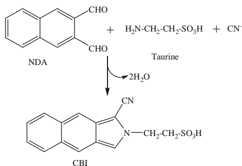
Fig. 1 Schematic representation of the reaction of NDA and taurine in the presence of cyanide to form an N-substituted 1-cyano[f]benzoinsole (CBI) complex
