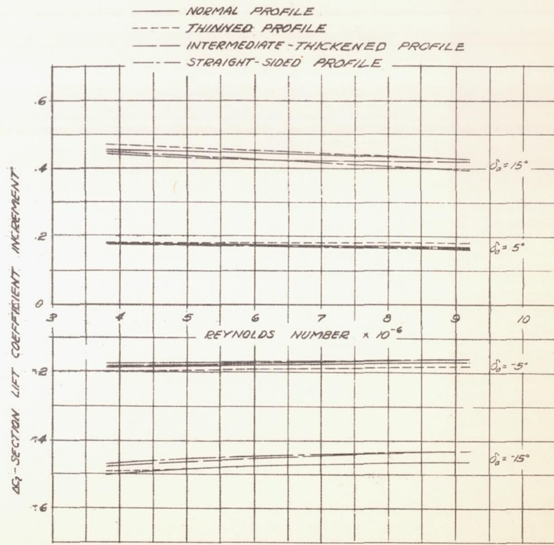
FIGURE 36.—THE EFFECT OF REYNOLDS NUMBER ON THE SECTION AERODYNAMIC CHARACTERISTICS OF AN NACA 65, 2-216 ( u = 0.6 ) AIRFOIL EQUIPPED WITH 0.15-CHORD, SEALED GAP, FLAT AILERONS. \alpha_{cr} = 0.01^\circ
