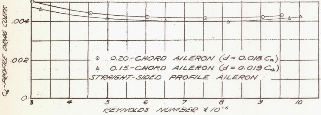
FIGURE 15.- THE EFFECT OF MODIFICATION OF THE AILERON PROFILE ON THE VARIATION OF SECTION PROFILE-DRAG COEFFICIENT WITH REYNOLDS NUMBER FOR AN NACA 66,2-216 ( \alpha=0.6 ) AIRFOIL. AILERON UNDEFLECTED. \alpha_0=0.51^\circ
