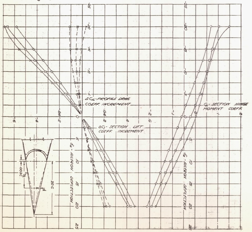
FIGURE 8b.- SECTION AERODYNAMIC CHARACTERISTICS OF AN NACA 66, 2-216 ( \alpha=0.6 ) AIRFOIL EQUIPPED WITH A 0.20-CHORD, SEALED GAP, PLAIN AILERON OF STRAIGHT-SIDED PROFILE, \alpha = 0.018 C_a .
