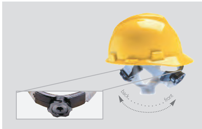
Swing-Ratchet Suspension
