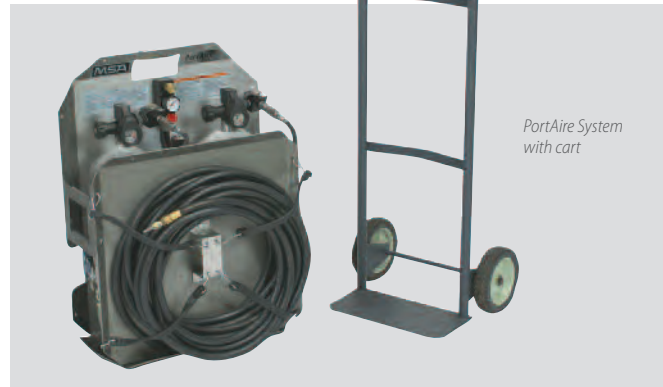
TransportAire System: High-Pressure Configuration
