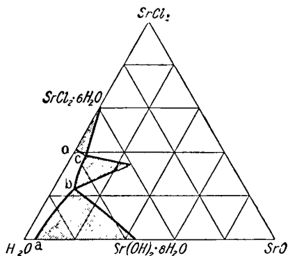
FIG. 15.—Ternary System, \text{SrO}-\text{SrCl}_2-\text{H}_2\text{O} , at 25^\circ .
