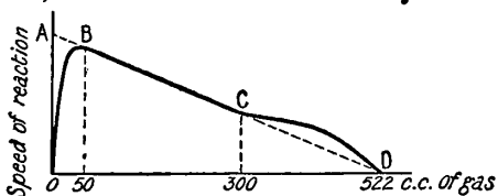
FIG. 56.—W. Spring's Diagram showing the Speed of the Reaction between Calcium Carbonate and Hydrochloric Acid.
