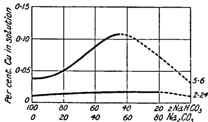
FIG. 38.—Per cent. of + and - Copper in Solutions of the Two Sodium Carbonates.
