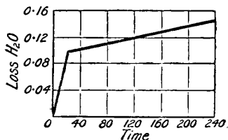
FIG. 13.—Velocity Curve of the Dehydration of \text{BaCl}_2 \cdot 2\text{H}_2\text{O} .
