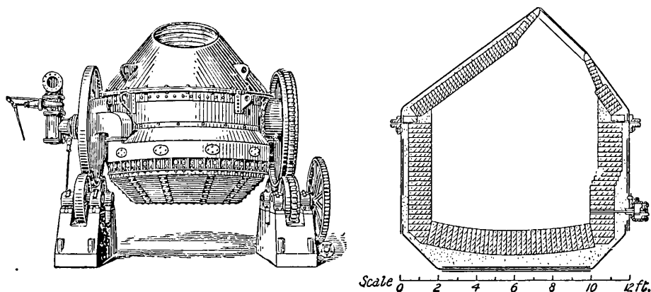
FIG. 8.—Converter.
