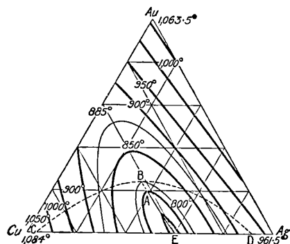
FIG. 20.—Isothermic Lines of Ternary Alloys of Copper-Silver-Gold.
