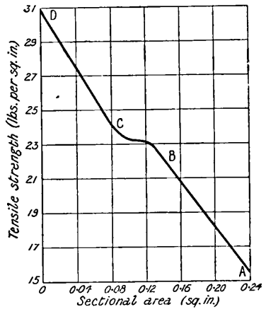
FIG. 11.—Effect of Sectional Area on the Tensile Strength of Copper Wire.
