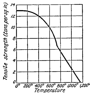
FIG. 12.—The Tensile Strength of Copper at different Temperatures.
