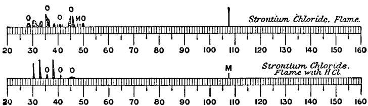
FIG. 4.—Flame Spectra of Strontium Chloride.
