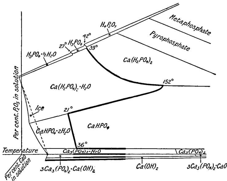
FIG. 63.—Equilibrium Conditions in the Ternary System, \text{CaO}-\text{P}_2\text{O}_5-\text{H}_2\text{O} , in the Region of the Orthophosphates—partly diagrammatic.
