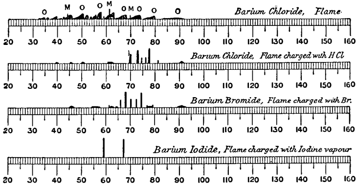
FIG. 5.—Flame Spectra of Barium Halides.
