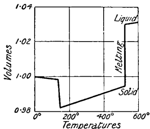
FIG. 16.—Relation between the Temperature and Volume of Silver Iodide.—(G. F. Rodwell.)
