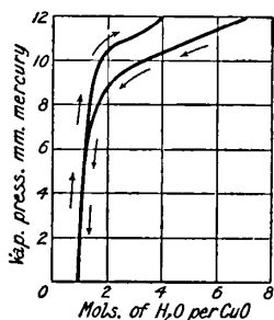
Fig. 25.—Hydration and Dehydration Curves of the Hydrogel of Cupric Oxide.
