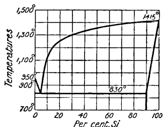
FIG. 13.—Fusion Curves of Alloys of Silver and Silicon.
