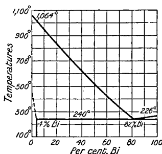
FIG. 8.—Fusion Curves of Mixtures of Gold and Bismuth.
