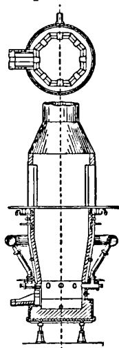
FIG. 2.—Cupola Furnace.
