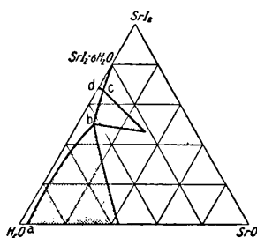
FIG. 36.—Ternary System, \text{SrI}_2 — \text{SrO} — \text{H}_2\text{O} , at 25^\circ .
