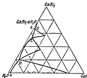
FIG. 23.—Ternary System, \text{CaBr}_2 — \text{CaO} — \text{H}_2\text{O} , at 25^\circ .
