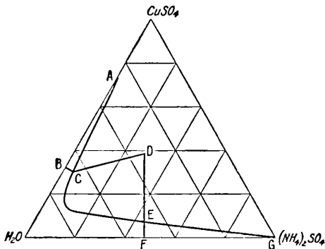
FIG. 36.—Equilibrium Curves in the Ternary System, \text{CuSO}_4 - (\text{NH}_4)_2\text{SO}_4 - \text{H}_2\text{O} , at 30^\circ .
