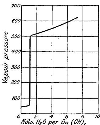
FIG. 10.—Vapour Pressure in the System \text{Ba}(\text{OH})_2\text{—H}_2\text{O} .
