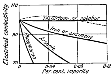
FIG. 17.—Effect of Impurities on the Electrical Conductivity of Copper.
