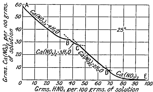
FIG. 60.—Equilibrium Conditions of the Ternary System, \text{Ca}(\text{NO}_3)_2-\text{HNO}_3-\text{H}_2\text{O} , at 25^\circ .
