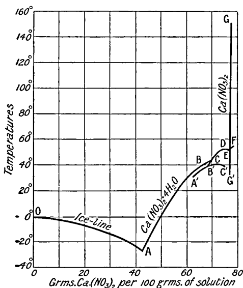
FIG. 59.—Solubility Curve of Calcium Nitrate.
