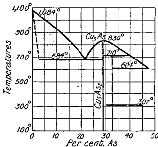
Fig. 18.—Freezing Point Curves of Copper-Arsenic Alloys.
