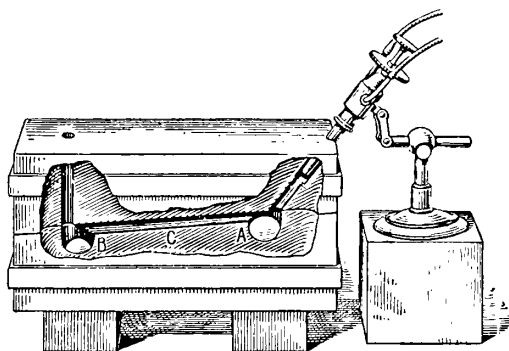
FIG. 6.—Apparatus for the Distillation of Silver.
