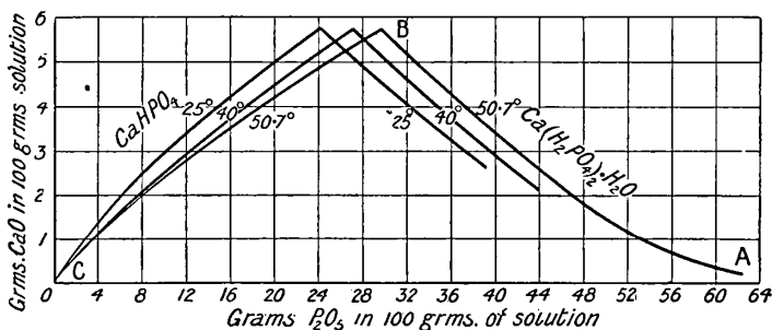
FIG. 67.—The Composition of Solutions in Equilibrium with Crystalline Calcium Hydro- and Dihydrophosphates.
