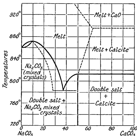
FIG. 57.—Fusion Curve of Binary Mixtures of Sodium and Calcium Carbonates.
