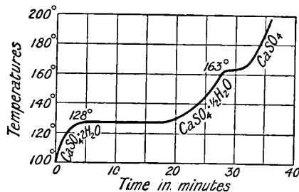
FIG. 38.—Heating Curve of Gypsum.
