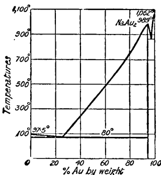
FIG. 16.—Freezing-point Curve of Sodium-Gold Alloys.
