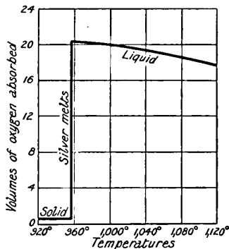
FIG. 9.—The Solubility of Oxygen in Silver.
