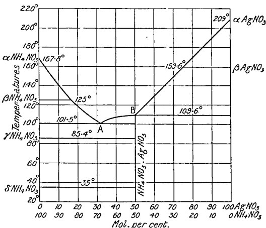
Fig. 26.—Fusion Curves of the Binary System, \text{AgNO}_3 - \text{NH}_4\text{NO}_3 (J. von Zawadsky).
