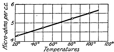
FIG. 7.—The Electrical Resistance of Calcium.
