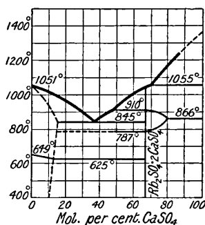
FIG. 48.—Fusion Curve of Calcium and Rubidium Sulphates.
