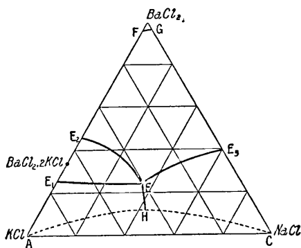
FIG. 22.—Ternary System, \text{BaCl}_2 — \text{KCl} — \text{NaCl} .
