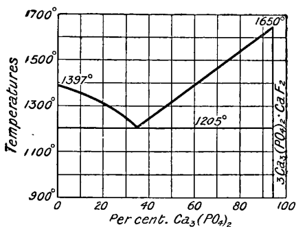
FIG. 68.—Fusion Curve of Mixtures of Calcium Phosphate and Fluoride.
