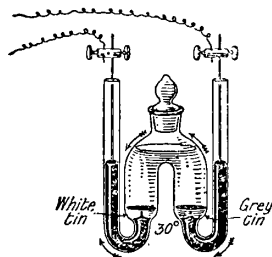
FIG. 22.—Electrical Method for Finding the Transition Point.
