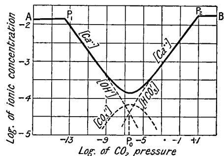
FIG. 55.—Relation between the Partial Pressure of Carbon Dioxide and the Concentrations of the several Ions in the System, \text{CaO}-\text{H}_2\text{O}-\text{CO}_2 , at 16°.
