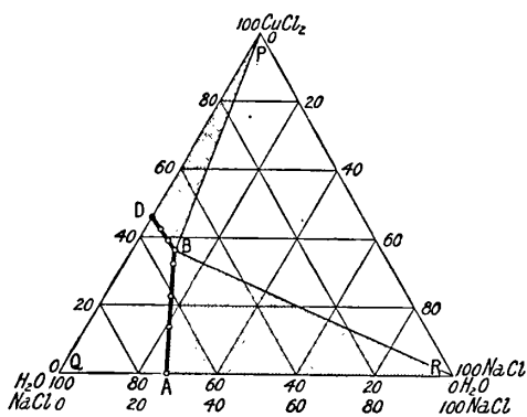
Fig. 29.—Equilibrium Diagrams for the Ternary System, \text{CuCl}_2 — \text{NaCl} — \text{H}_2\text{O} , at 30^\circ .
