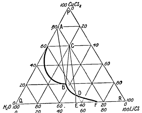
FIG. 28.—Equilibrium Diagram for the Ternary System, \text{CuCl}_2 - \text{LiCl} - \text{H}_2\text{O} , at 30^\circ .
