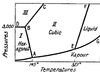
FIG. 15.—Equilibrium Diagram of Silver Iodide.
