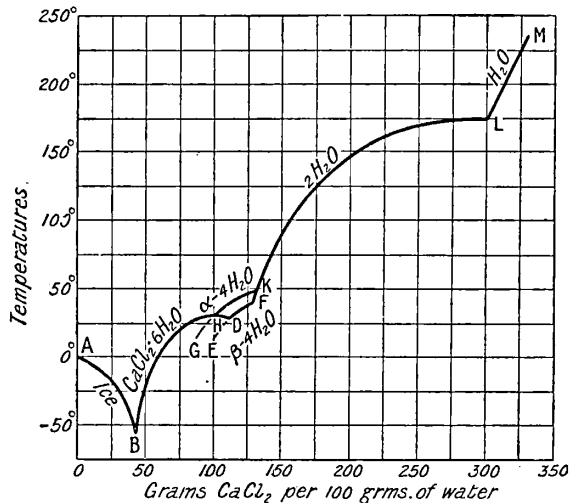
FIG 12.—Solubility Curve of Calcium Chloride
