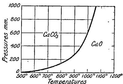
Fig. 9.—Effect of Temperature on the Dissociation Pressure of Calcium Carbonate.
