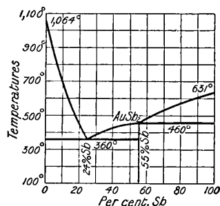
FIG. 7.—Fusion Curves of Mixtures of Gold and Antimony.
