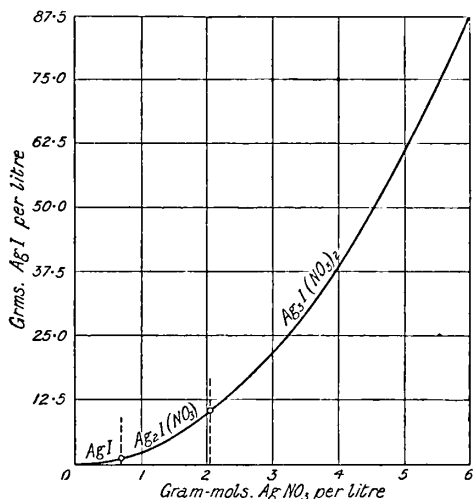
FIG. 25.—Solubility of Silver Iodide in Solutions of Silver Nitrate.
