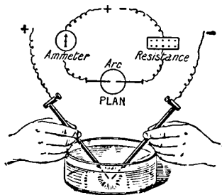
FIG. 12.—G. Bredig's Method of making Metal Sols by the Direct Current Arc.
