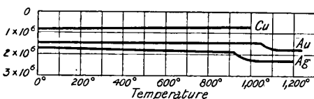
FIG. 8.—Magnetic Susceptibility of Copper, Silver, and Gold at different Temperatures.
