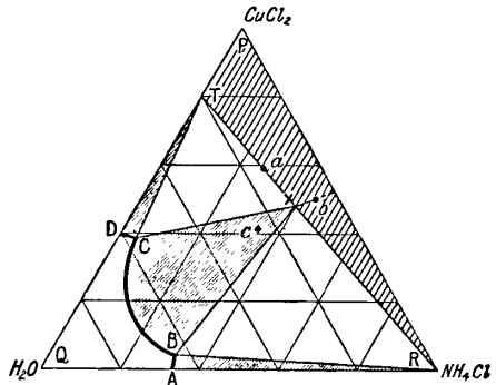
FIG. 30.—Equilibrium Curves for Ternary Systems, \text{CuCl}_2 — \text{NH}_4\text{Cl} — \text{H}_2\text{O} . at 30°.
