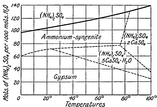
FIG. 52.—Equilibrium Concentration of Ammonium Sulphate for the different Solid Phases with Calcium Sulphate.
