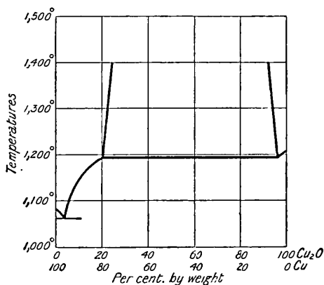
FIG. 24.—Fusion Curve of Mixtures of Copper and Cuprous Oxide.
