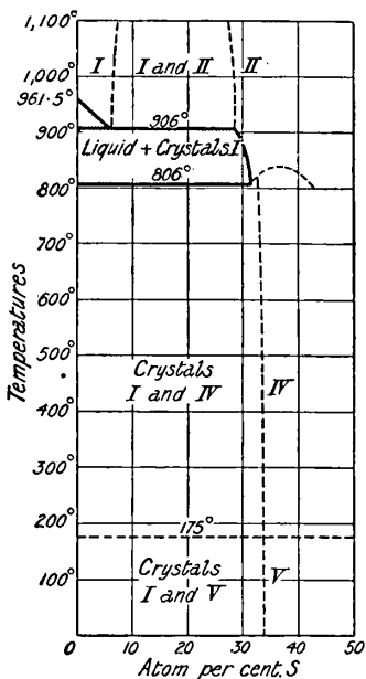
FIG. 19.—Equilibrium Curve of Binary Mixtures of Sulphur and Silver.
