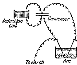
FIG. 13.—T. Svedberg's Method of making Colloidal Metals by the Oscillatory Discharge.
