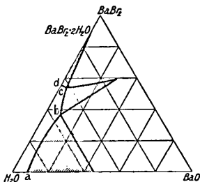
FIG. 25.—Ternary System, \text{BaBr}_2 - \text{BaO} - \text{H}_2\text{O} , at 25^\circ .
