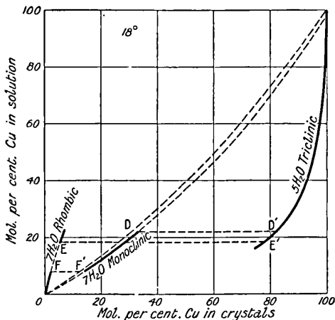
FIG. 35.—Relation between Copper and Zinc in the Mixed Crystals and in the Soln.
