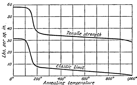
FIG. 9.—The Effect of Annealing at different Temperatures on the Tensile Strength and Elastic Limit of Electrolytic Copper (C. Grard).
