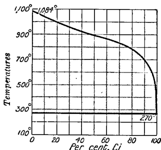
FIG. 20.—Freezing Point Curves of Copper-Bismuth Alloys.
