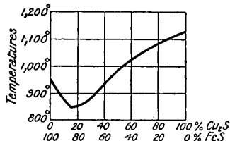
FIG. 4.—Freezing Curve of Mixtures of Ferrous and Cuprous Sulphides.
