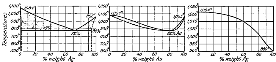
FIG. 17.—Freezing-point Curves of Copper-Silver Alloys. FIG. 18.—Freezing-point Curves of Copper-Gold Alloys. FIG. 19.—Freezing-point Curve of Gold-Silver Alloys.
