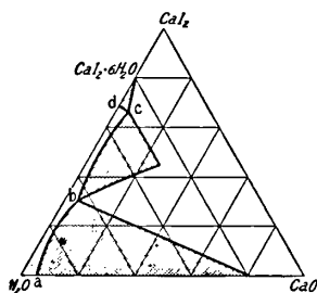
FIG. 35.—Ternary System, \text{CaI}_2 — \text{CaO} — \text{H}_2\text{O} , at 25^\circ .
