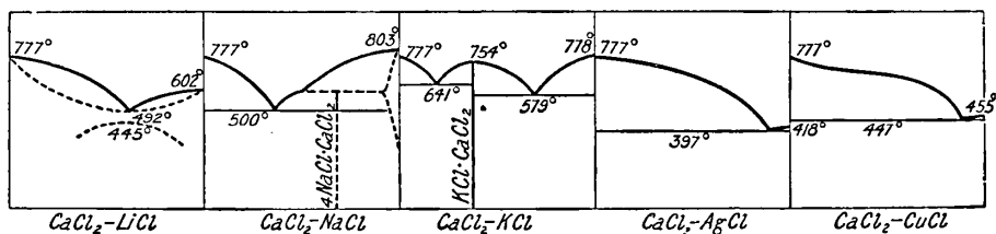
FIGS. 16 to 20.—Freezing-point Curves of Binary Mixtures of Calcium Chloride with Lithium, Sodium, Potassium, Cuprous, and Silver Chloride.
