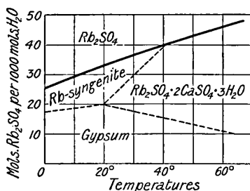
FIG. 51.—Equilibrium Concentration of Rubidium Sulphate for the different Solid Phases with Calcium Sulphate.
