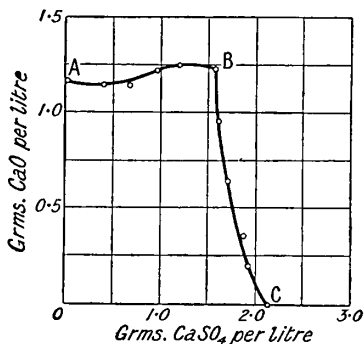
FIG. 45.—Mutual Solubility of Calcium Oxide and Sulphate in Water at 25°.
