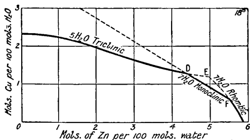
FIG. 34.—Limiting Range in Composition of Soln. for Mixed Crystals of Copper and Zinc Sulphates.
