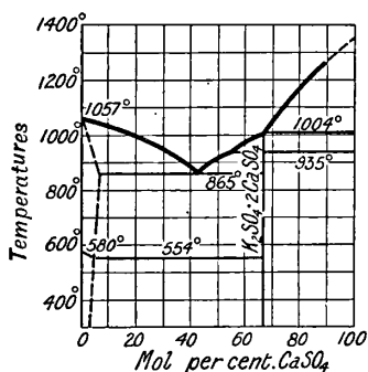
FIG. 47.—Fusion Curve of Calcium and Potassium Sulphates.
