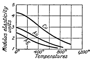
FIG. 10.—Effect of Temperature on the Modulus of Elasticity.
