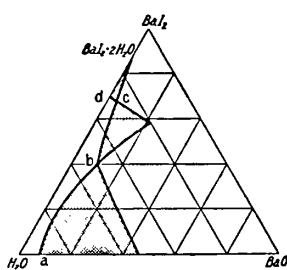
FIG. 37.—Ternary System, \text{BaI}_2 — \text{BaO} — \text{H}_2\text{O} , at 25^\circ .
