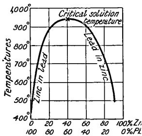
FIG. 5.—Mutual Solubility of Lead and Zinc.
