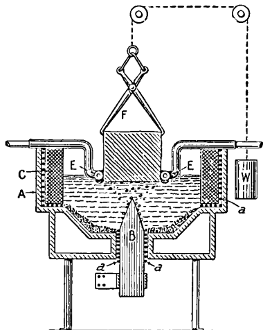
FIG. 1.—G. O. Seward and F. von Kugelgen's Electrolytic Cell for Calcium.
