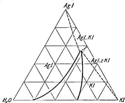
FIG. 18.—Equilibrium Curves in the Ternary System, AgI—KI—H 2 O at 50°
