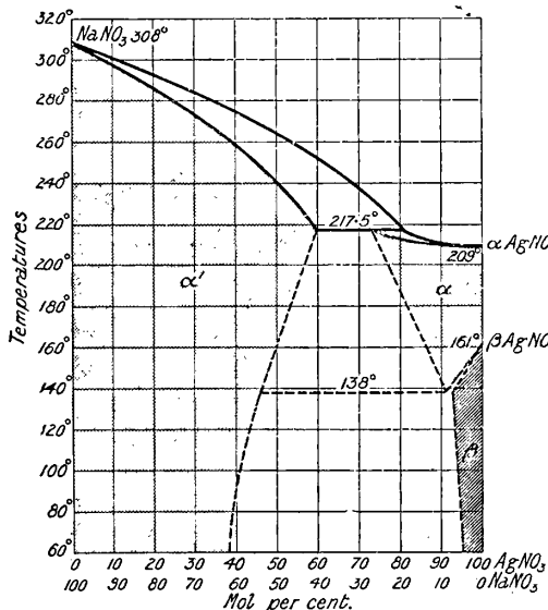
FIG. 28.—Fusion Curves of the Binary System, \text{NaNO}_3\text{—AgNO}_3 (D. J. Hissink).
