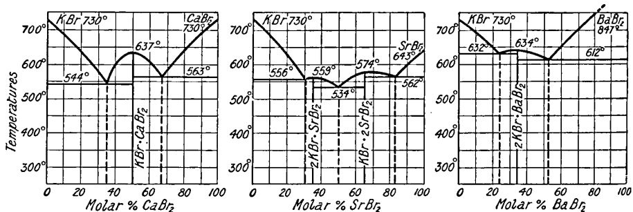
FIGS. 32 TO 34.—Freezing-point Curves of Binary Mixtures of Potassium Bromide with Calcium, Strontium, and Barium Bromides.
