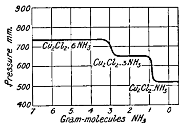
FIG. 26.—Vapour Pressure Curves of the Cuprous Ammino-chlorides.
