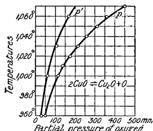
FIG. 23.—Dissociation Pressures, 2\text{CuO} \rightleftharpoons \text{Cu}_2\text{O} + \text{O}_2 .
