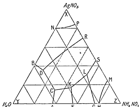
FIG. 27.—Ternary System, \text{NH}_4\text{NO}_3\text{—AgNO}_3\text{—H}_2\text{O} (Diagrammatic).
