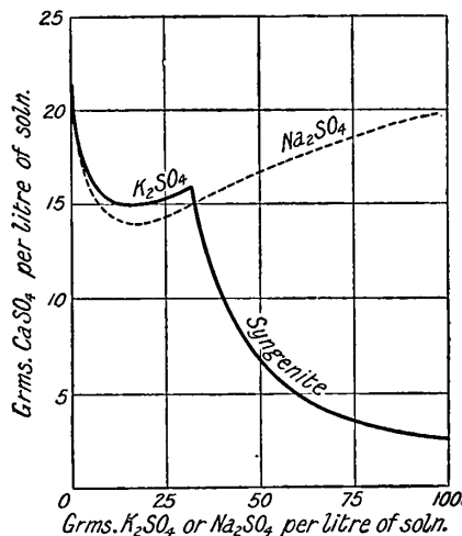
FIG. 49.—Solubility of Calcium Sulphate in Soln. of Potassium and Sodium Sulphates.
