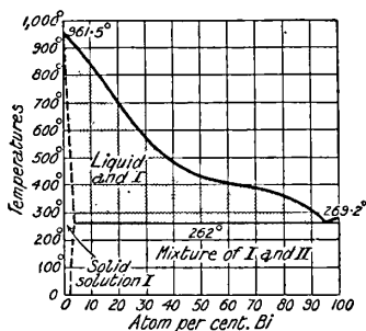
FIG. 12.—Freezing Point Curve of Silver-Bismuth Alloys (G. I. Petrenko).
