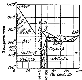
Fig. 19.—Freezing Point Curves of Copper-Antimony Alloys.
