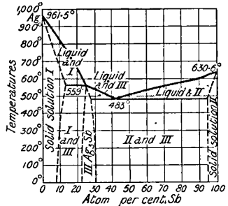
Fig. 11.—Freezing Point Curve of the Binary System Ag-Sb (G. I. Petrenko).
