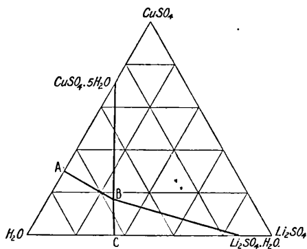
FIG. 37.—Equilibrium Curves of the Ternary System, \text{Li}_2\text{SO}_4\text{—CuSO}_4\text{—H}_2\text{O} , at 30^\circ .
