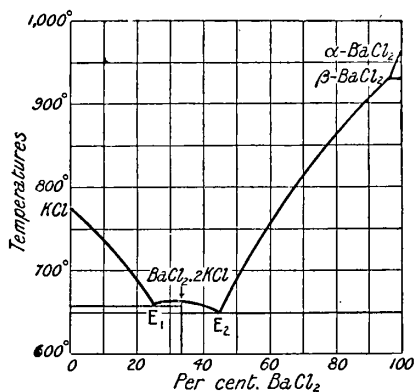
FIG. 21.—Melting-point Curve of Binary Mixtures, \text{BaCl}_2 — \text{KCl} .
