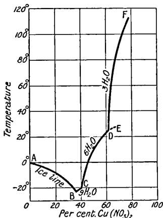
FIG. 39.—Solubility Curve of Cupric Nitrate.
