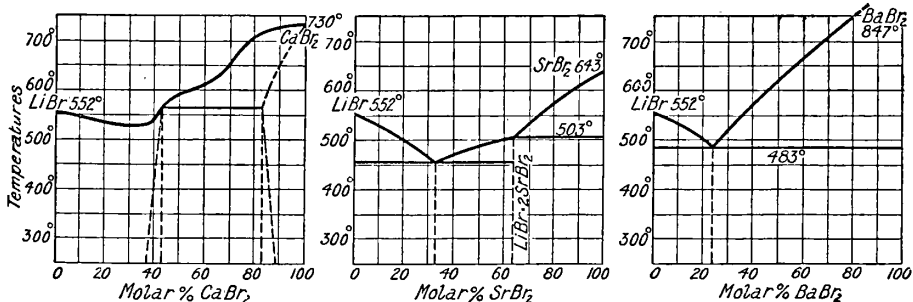
FIGS. 26 TO 28.—Freezing-point Curves of Binary Mixtures of Lithium Bromide with Calcium, Strontium, and Barium Bromides.
