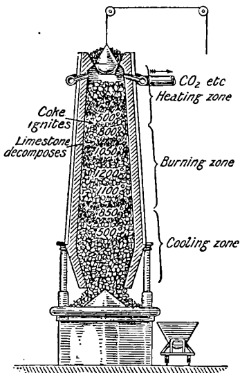
FIG. 8.—Simple Type of Shaft Lime-kiln.
