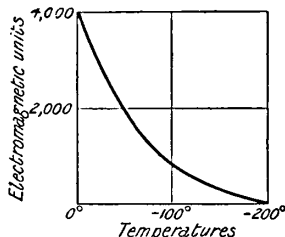
FIG. 16.—Effect of Low Temperature on Electrical Resistance of Copper.
