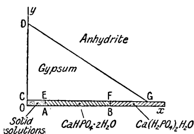
FIG. 64.—Phases of the Four Component System: \text{CaO}-\text{H}_3\text{PO}_4-\text{H}_2\text{SO}_4-\text{H}_2\text{O} .
