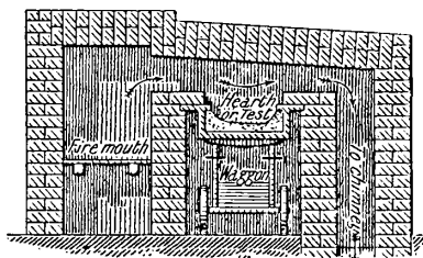
FIG. 2.—Diagrammatic Section of the English Cupellation Furnace.
