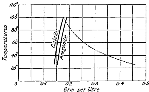
FIG. 54.—Solubility of Calcite and Aragonite in Water.
