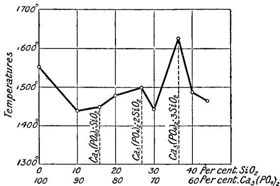
FIG. 65.—Fusion Temperatures of Mixtures of Silica and Normal Calcium Phosphate.
