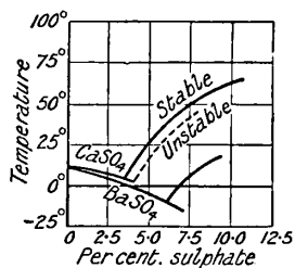
FIG. 42.—Freezing-point Curves of Binary Mixtures of Sulphuric Acid with Barium or Calcium Sulphate.
