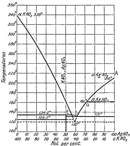
FIG. 29.—Fusion Curves of the Binary System, \text{KNO}_3 - \text{AgNO}_3 (A. Ussoff).
