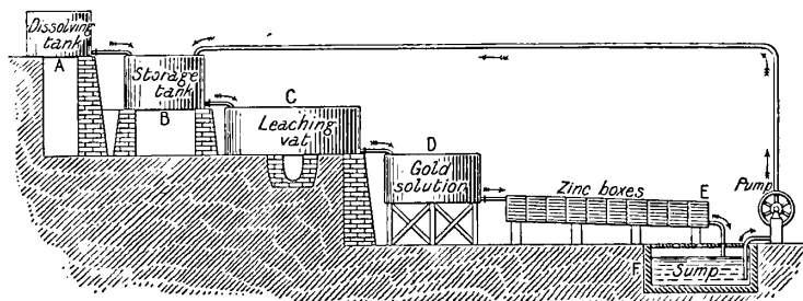
FIG. 4.—Diagrammatic Representation of Cyanide Plant.
