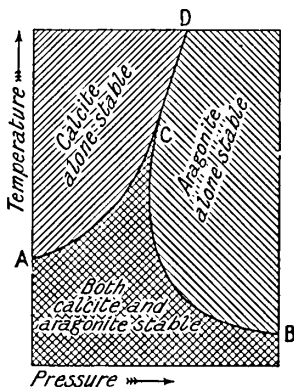
FIG. 53.—Zones of Stability of Calcite and Aragonite.
