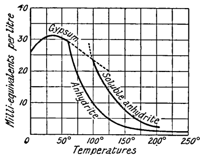
FIG. 41.—Solubility of Calcium Sulphate in Water.
