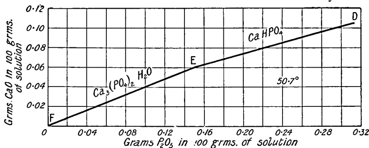
FIG. 66.—The Composition of Solutions in Equilibrium with Crystalline Calcium Hydrophosphate, and with Monohydrated Normal Calcium Phosphate.
