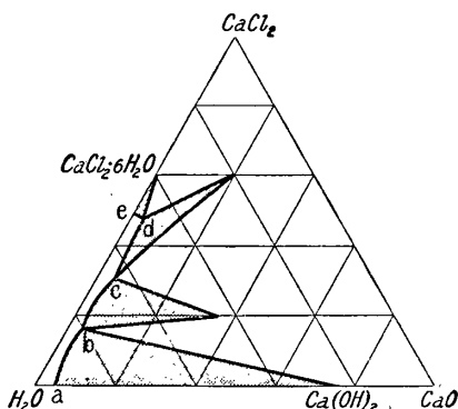
FIG. 14.—Ternary System, \text{CaO}-\text{CaCl}_2-\text{H}_2\text{O} , at 10^\circ .
