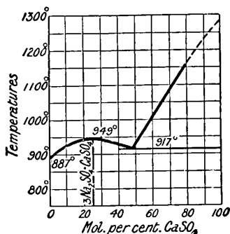
FIG. 46.—Fusion Curve of Calcium and Sodium Sulphates.
