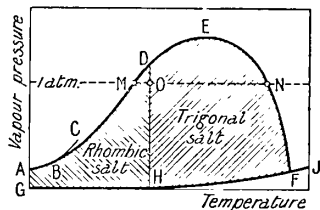
FIG. 24.—Meyerhoffer's Vapour Pressure Curves of Solutions of Silver Nitrate. (Diagrammatic.)
