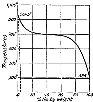
FIG. 15.—Freezing-point Curve of Sodium-Silver Alloys.
