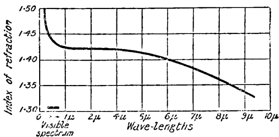
FIG. 11.—Dispersion Curve of Fluorite.
