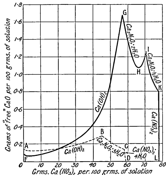
FIG. 61.—Equilibrium Curves in the Ternary System, \text{CaO}-\text{Ca}(\text{NO}_3)_2-\text{H}_2\text{O} , at 25° and at 100°.
