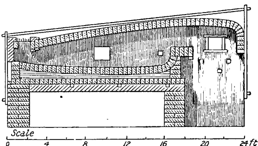
FIG. 7.—Reverberatory Furnace.
