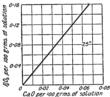
FIG. 70.—Isothermal Solubility Curve for Basic Calcium Phosphate.
