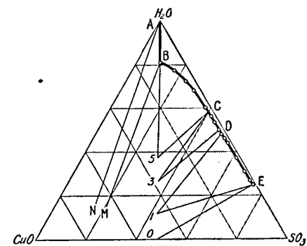
FIG. 33.—Ternary System, CuO—SO 3 —H 2 O, at 25°.
