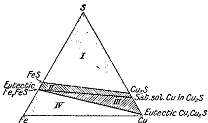
FIG. 3.—Triangular Diagram for Ternary Mixtures of Copper, Iron, and Sulphur.
