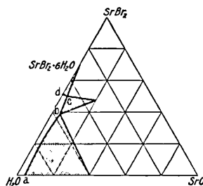
FIG. 24.—Ternary System, \text{SrBr}_2 — \text{SrO} — \text{H}_2\text{O} , at 25^\circ .
