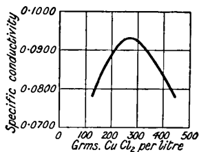
FIG. 27.—Specific Conductivity and Concentration Curve of \text{CuCl}_2 .
