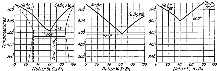
FIGS. 29 TO 31.—Freezing-point Curves of Binary Mixtures of Sodium Bromide with Calcium, Strontium, and Barium Bromides.
