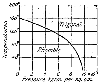
FIG. 23.—Effect of Pressure on the Transition Point of Silver Nitrate.
