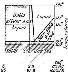
FIG. 4.—The Eutectic Portion of Freezing Curve of Silver-Lead Alloys.
