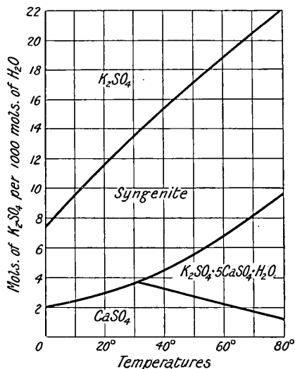
FIG. 50.—Equilibrium Concentration of Potassium Sulphate for the different Solid Phases with Calcium Sulphate.
