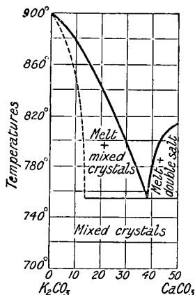
FIG. 58.—Fusion Curve of Binary Mixtures, \text{K}_2\text{CO}_3—\text{CaCO}_3 .
