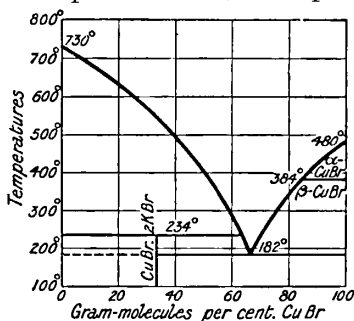
FIG. 32.—Fusion Curves of the Binary mixtures, KBr—CuBr.
