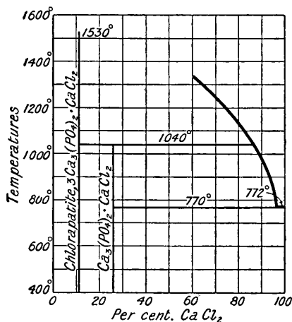
FIG. 69.—Fusion Curve of Mixtures of Calcium Phosphate and Chloride.
