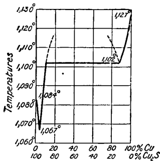
FIG. 6.—Freezing Curve of Mixtures of Copper and Cuprous Sulphide.
