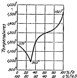
FIG. 5.—Freezing Curve of Mixtures of Iron and Ferrous Sulphide.
