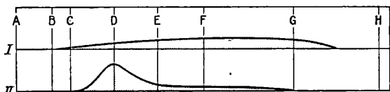
FIG. 14.—Action of different parts of the Spectrum on I. Silver Chloride alone; II. Silver Chloride with Coralline.
