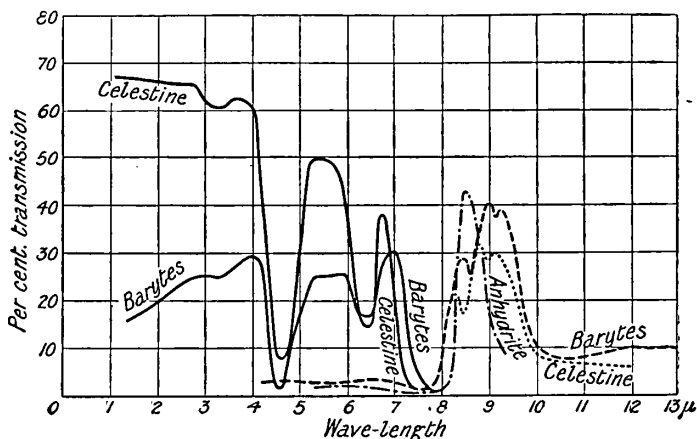
FIG. 44.—Absorption Spectra of Barytes and Celestine.
