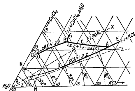
FIG. 31.—Equilibrium Curves of Portion of the Ternary System, \text{CuCl}_2 — \text{KCl} — \text{H}_2\text{O} , between -25^{\circ} and 100^{\circ} .
