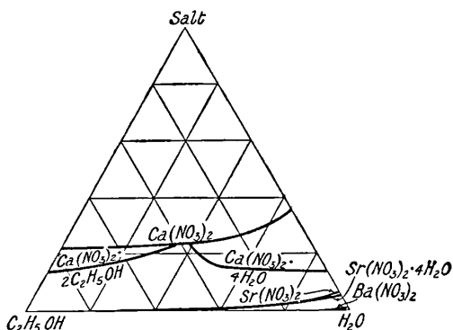
FIG. 62.—Equilibrium Diagram for the Ternary Systems, \text{M}(\text{NO}_3)_2 — \text{C}_2\text{H}_5\text{OH} — \text{H}_2\text{O} .
