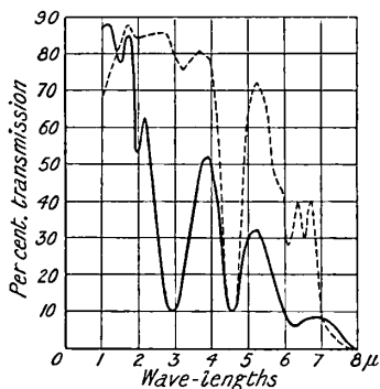
FIG. 43.—Absorption Spectra of Selenite and Anhydrite.
