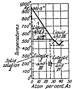
Fig. 10.—Freezing Point Curve of the Binary System Ag-As (K. Friedrich and A. Leroux).
