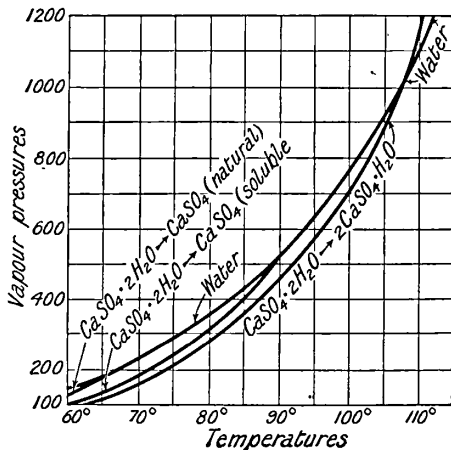
FIGS. 39 and 40.—Vapour Pressure Curves of the Hydrates of Calcium Sulphate.
