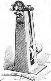
Felly Rounder.
