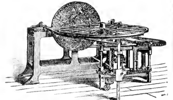
Wheel Tread Sander.
