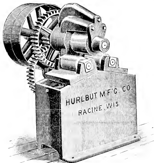
TIRE MACHINE.
