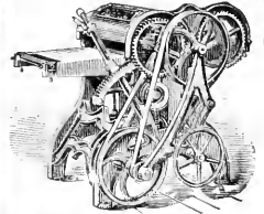
24-Inch Surfacers.
