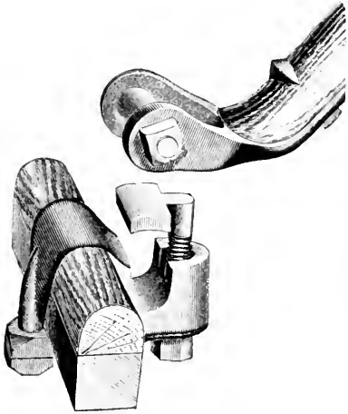
Coupling with shaft eye removed.
