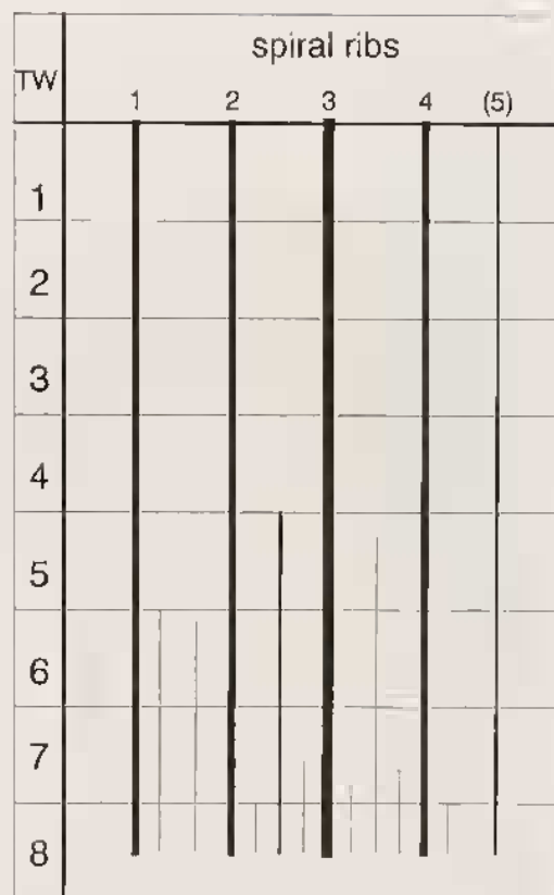
FIG. 74. — Mathilda richeri sp. nov. Diagram of spiral sculpture (holotype), as in Fig. 8.
