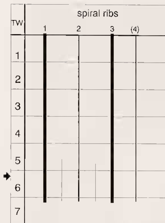
FIG. 8. — Mathilda brevicuda . Diagram of spiral sculpture, showing relative position and strength of exposed spiral ribs on the upper side of teleoconch whorls (TW). Rib number in parentheses indicates primary spiral rib serving as attachment of subsequent whorl. Arrow indicating condition of holotype.
