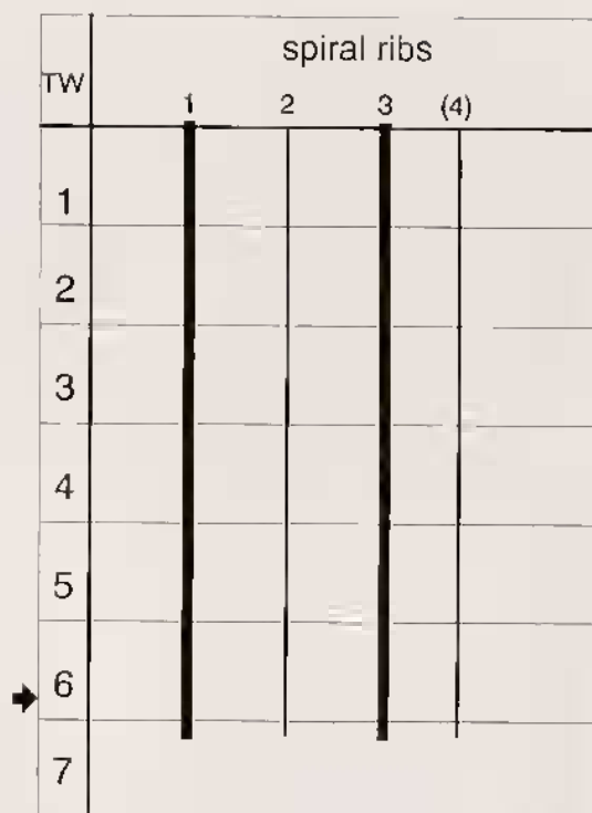
FIG. 9. — Mathilda bouchei sp. nov. Diagram of spiral sculpture, as in Fig. 8.
