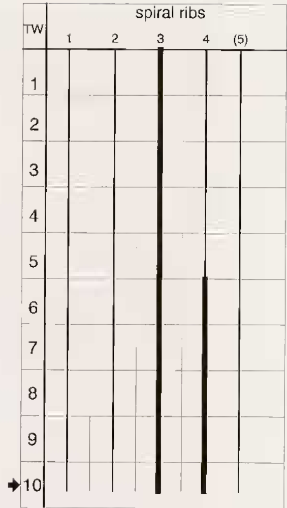
FIG. 39. — Mathilda salve . Diagram of spiral sculpture, as in Fig. 8. Fifth rib exposed in holotype.
