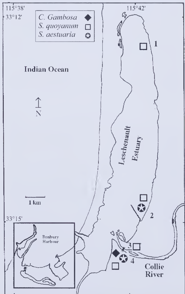
Figure 1. Distribution of sphaeromatid isopods in Leschenault Estuary and Collie River.
