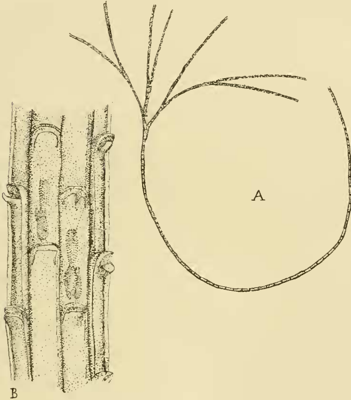
FIG. 4.— Farciminaria andamanensis , sp. nov. A. Habit sketch. \times 2 . B. A few zoecia. \times 50 .
