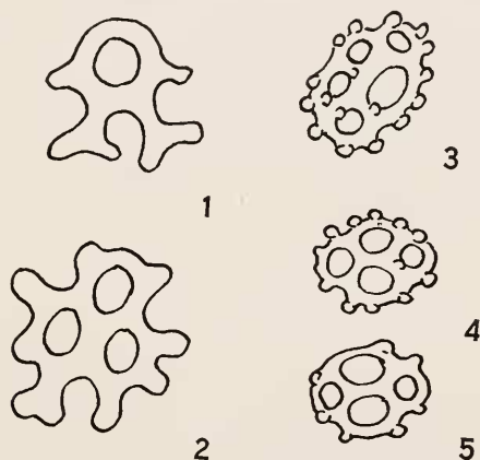
Figs. 1-2. Deposits from sole of Psolus squamatus Düben and Koren.
