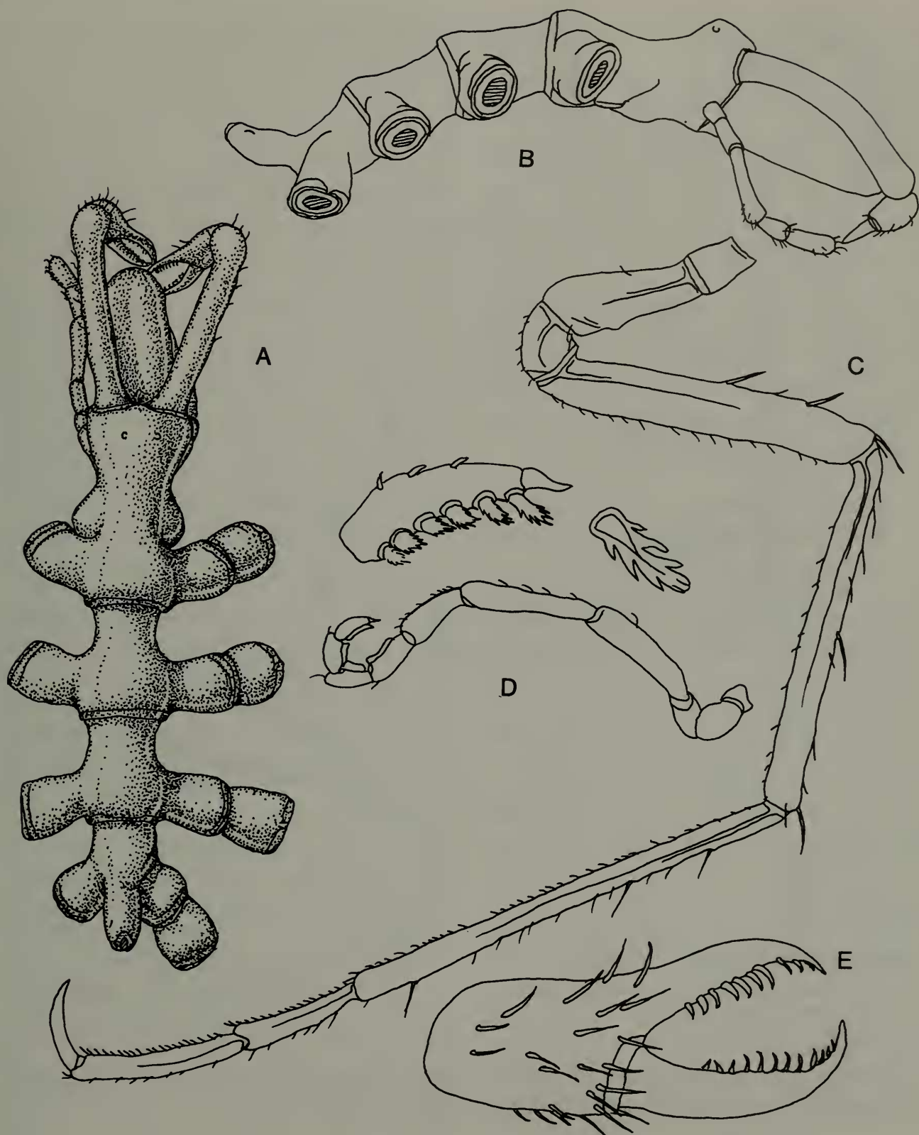
Fig. 1. Heteronymphon caecigenum , new species, holotype: A, Trunk, dorsal view; B, Trunk, lateral view; C, Third leg; D, Oviger, with enlargements of terminal segment and denticulate spine; E, Chela.
