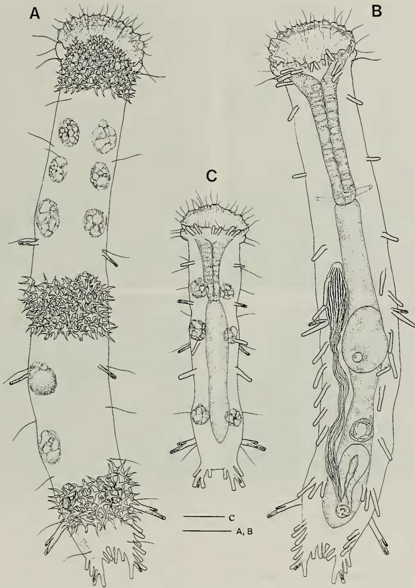
Fig. 1. Tetranchyroderma schizocirratum , new species: A, habitus, dorsal view; B, habitus, ventral view; C, habitus, juvenile, ventral view. Scale bars = 20 \mu\text{m} .
