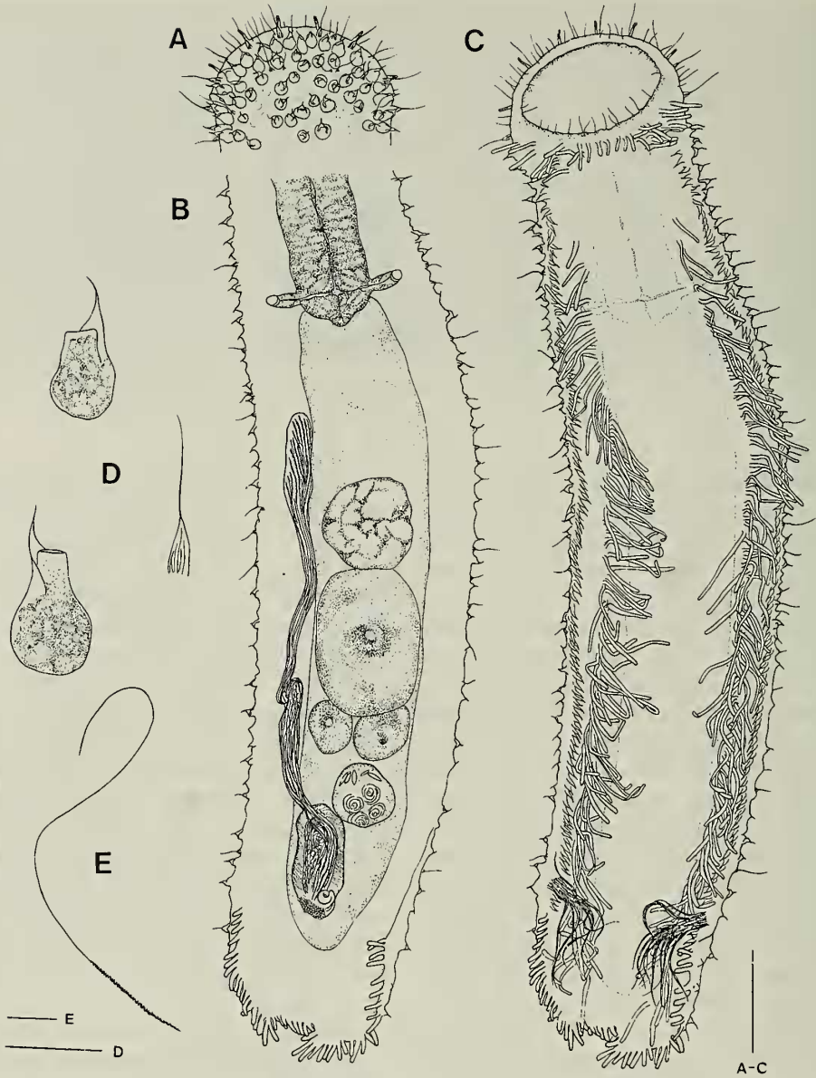
Fig. 5. Platydasys itoi , new species: A, head, dorsal view showing papillary armature; B, remainder after head, ventral view showing internal organs; C, habitus, ventral view; D, dorsal papillae; E, spermatozoon. Scale bars: A-C = 50 \mu\text{m} ; D, E = 10 \mu\text{m} .
