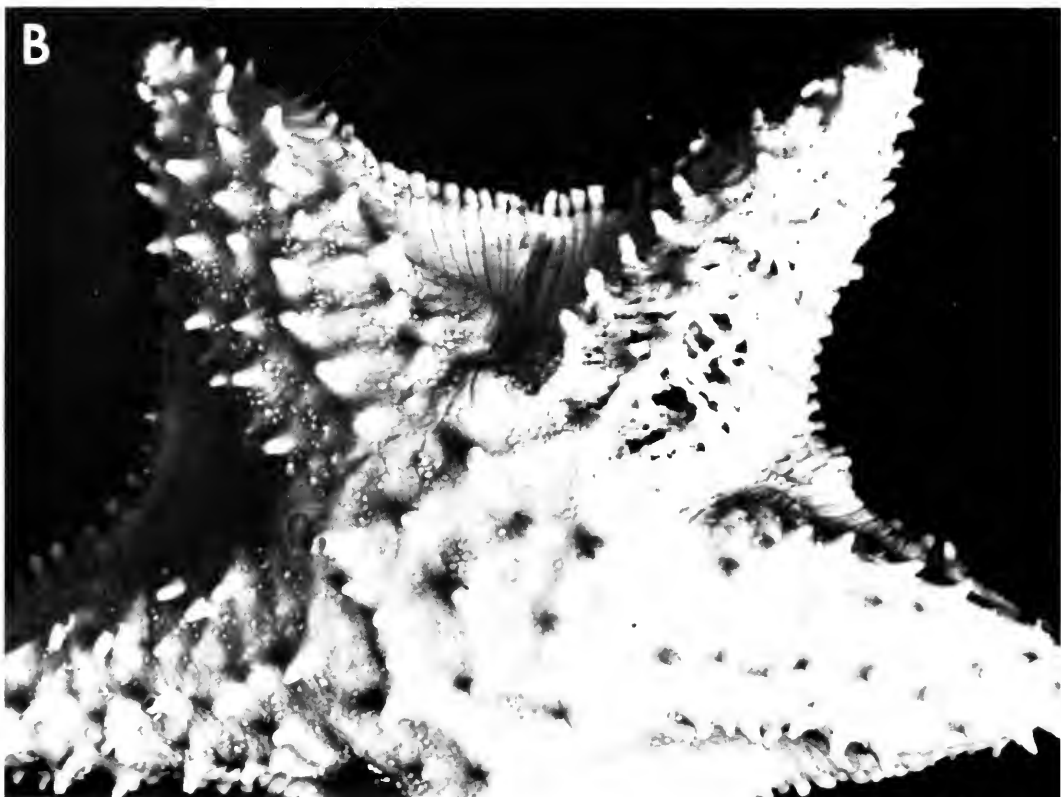
Fig. 1 A. Poramopsis echinaster Perrier, BM reg. no. 1975.11.12.9, Chinquihue, S Chile, R 36 mm; dry, partly denuded, showing spinules between the spines. \times 2 . B. Porania (Porania) antarctica magellanica Studer, 1948.3.16.448. Discovery Investigations st. 80, Falkland Is, R 60 mm; wet, showing papulae between the spines, the spinules microscopic. \times 1\frac{1}{2} .
