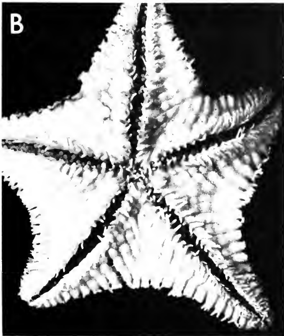
Fig. 2 A, Poraniopsis echinaster (as in 1A), partly denuded. \times 2 . B, Porania (Porania) pulvillus (O. F. Müller), 1922.4.10.1, Lousy Bank, SW of Faeroe Is, R c. 36 mm; wet but contracted, the contours of the plates showing their limits. \times 1\frac{1}{2} . C, Poraniella echinulata (Perrier), Pillsbury st. 853, Windward Is, R 10 mm; dry, partly denuded. \times 3 .
