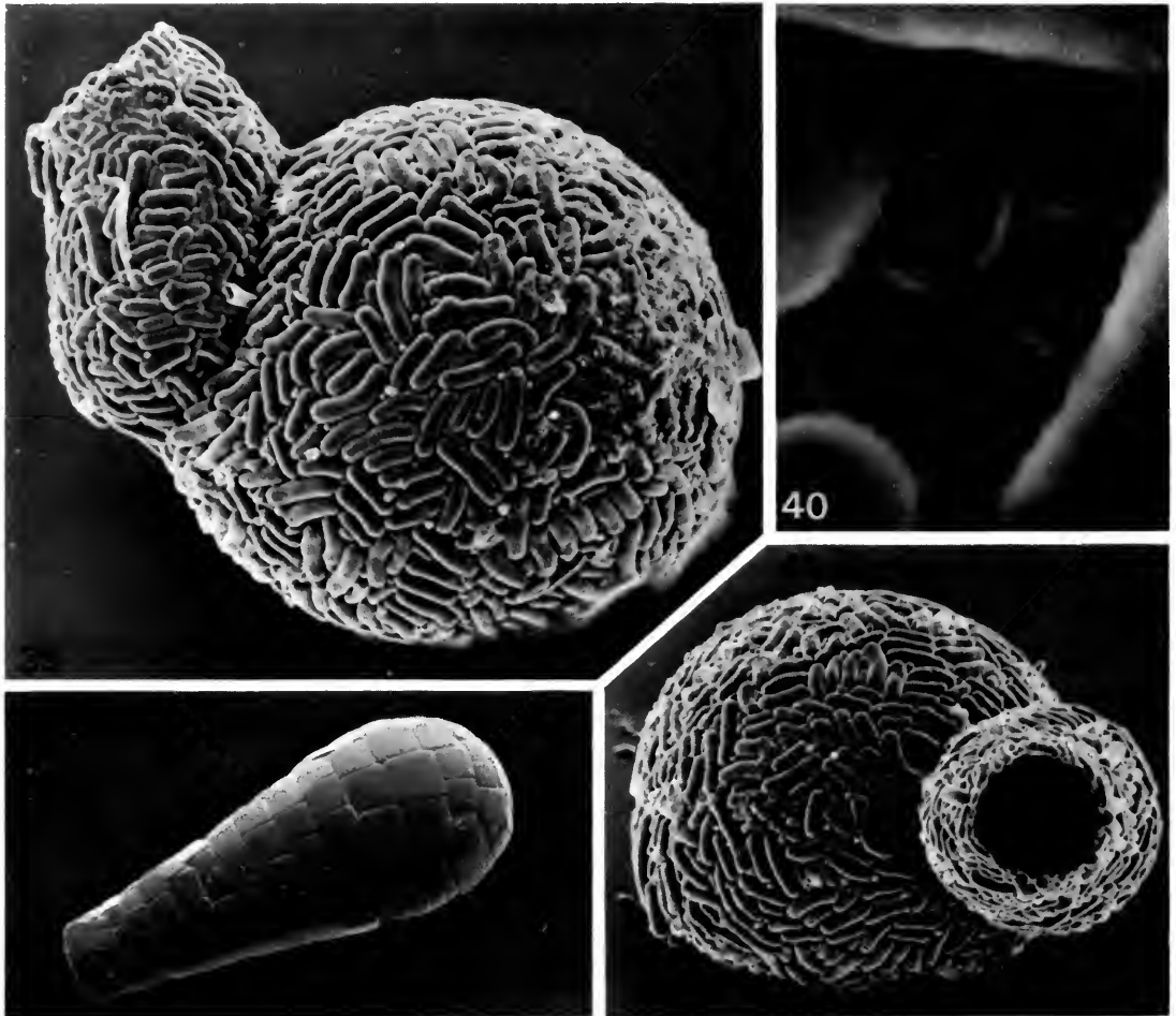
Figs 39–41 Lesquereusia epistomium : Fig. 39, lateral view, note the distinct neck \times 700 ; Fig. 40, detail of organic cement \times 25000 ; Fig. 41, apertural view \times 700 . Fig. 42 , Quadrullella symmetrica : lateral view of elongate specimen \times 500 .
