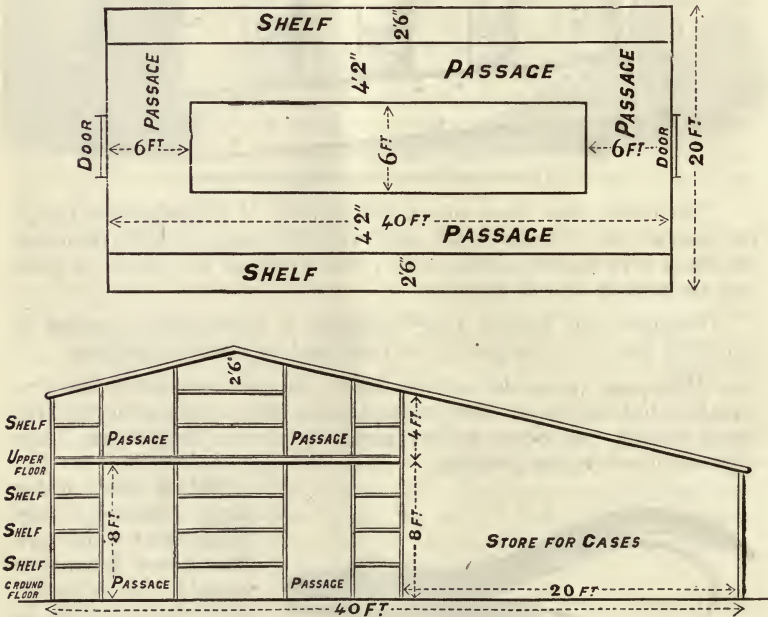
Fruit Storage House.
