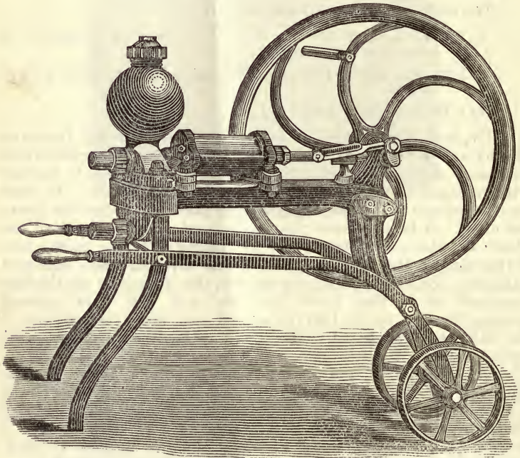
Wine Pump.
