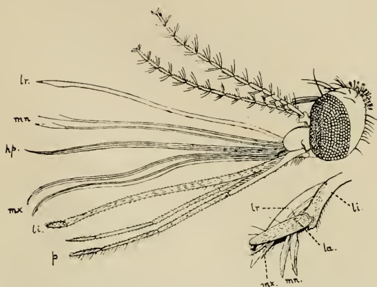
Fig. 363—PROBOSCIS OF FEMALE ANOPHELES (AFTER NUTTALL AND SHIPLEY). LR. LABRUM. MN. MANDIBLES. HP. HYPOPHARYNX. MX. MAXILLA. LI. LABIUM. LA. LABELLA. P. PALPI.
