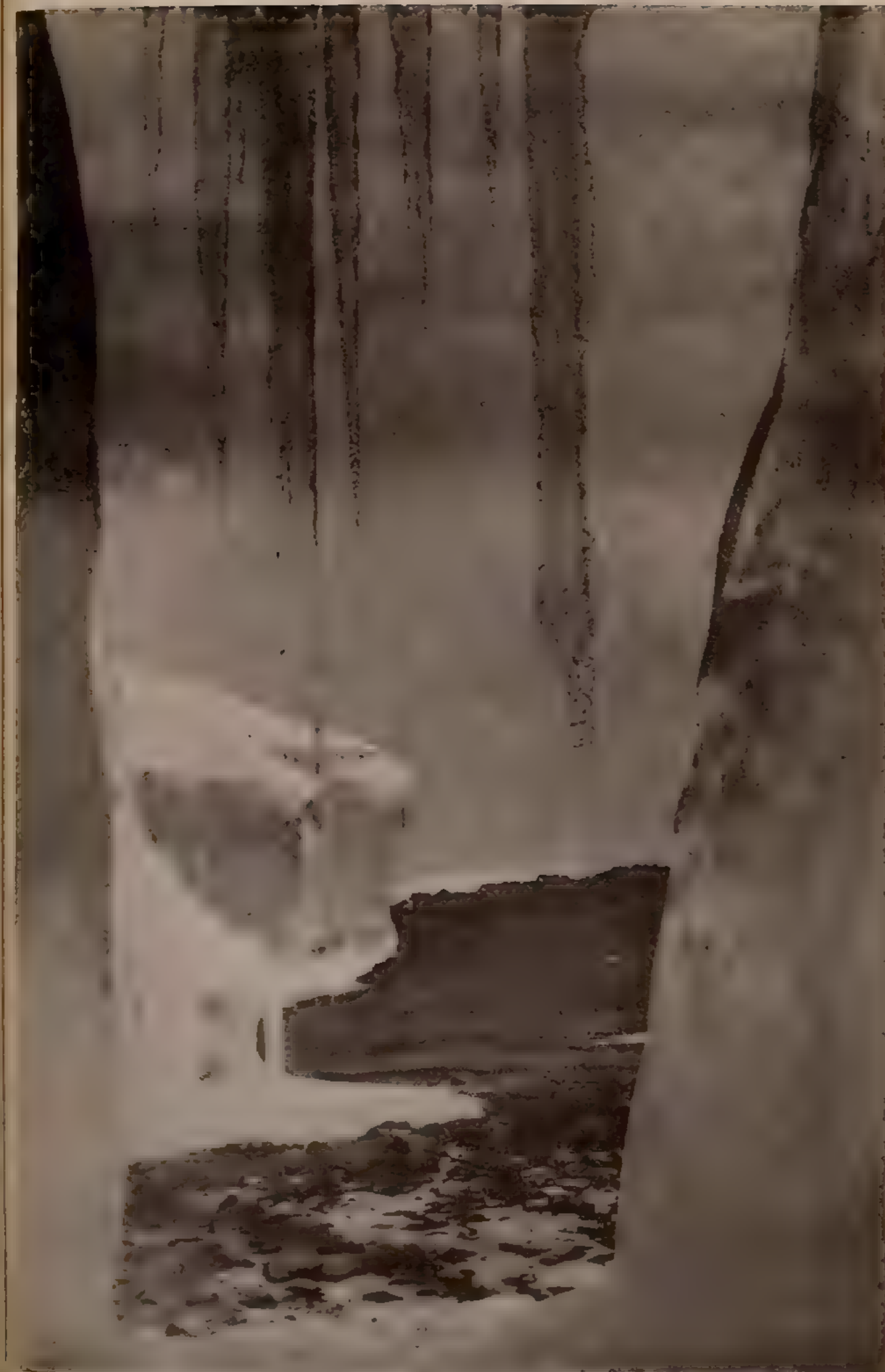
Fig. 19. Ice formations on Kibo along the Northern Ice Wall.
