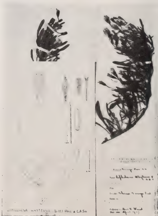
Fig. 5. Lopholaena Whyteana (Britt.) Phill. at C.A.S.
