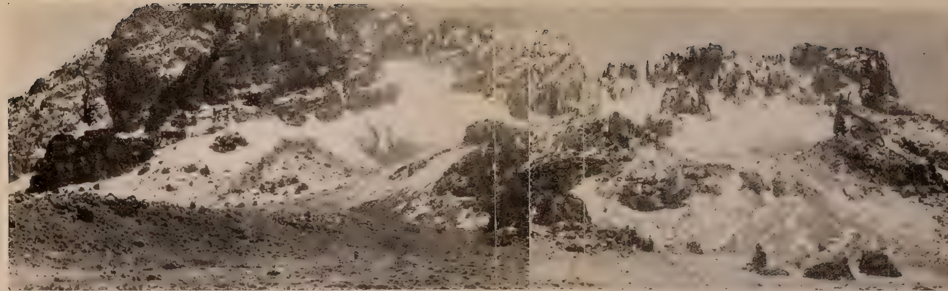
Fig. 2. The massif of Mawenzi from the saddle.
