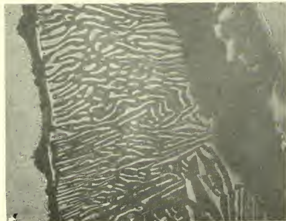
FIG. 1.—Part of area in pl. 22, fig. 2, at high magnification. The dark lamellae are shown to be not tacinite but kamacite, invaded by hydroxide and wholly altered; the tacinite, resistant to oxidation, surrounding hydroxide. Pical 15 seconds; \times 300.
