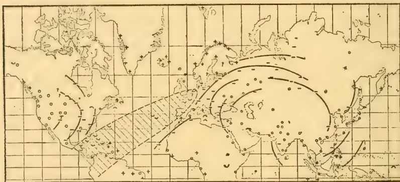
FIG. 23.—Pressure differences for September and October.
