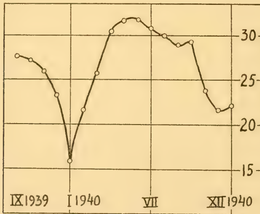
FIG. 22.—Temperature differences, 6 km. and surface, Omaha, Nebr.
