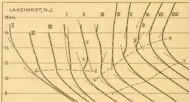
FIG. 18.—The tropopause at Lakehurst, N. J.
