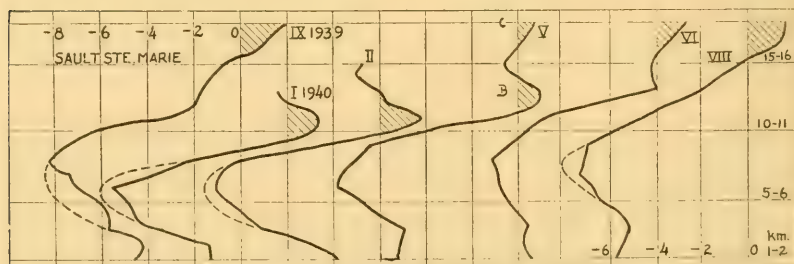
FIG. 14.—Lapse rates of temperature, Sault Ste. Marie.
