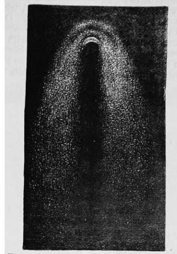
FIG. 1.—Head and Envelopes of a Comet.
