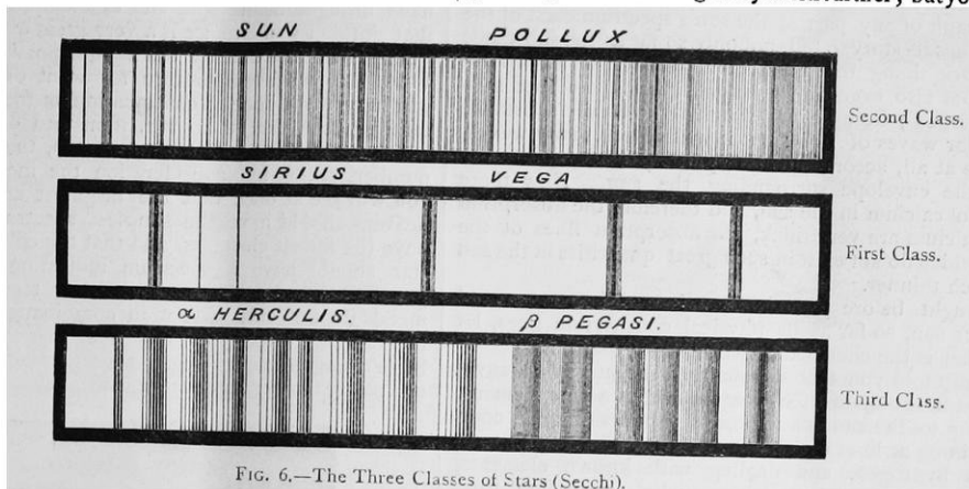
FIG. 6.—The Three Classes of Stars (Secchi).
