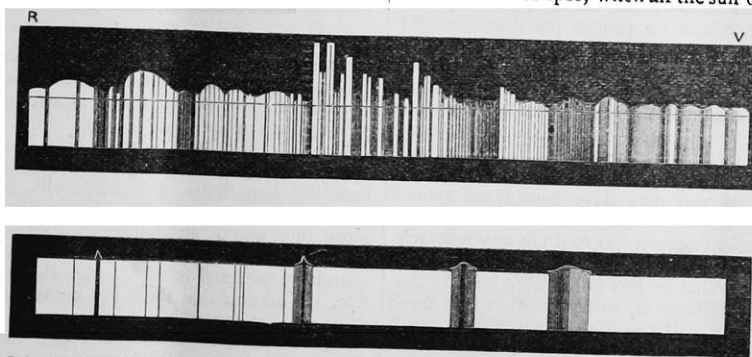
FIG. 7.—Spectra of \alpha Orionis and Sirius (Secchi). In the spectrum of \alpha Orionis the brightness of the spectrum is represented by the height.
