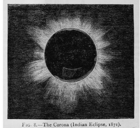
FIG. 8.—The Corona (Indian Eclipse, 1871).
