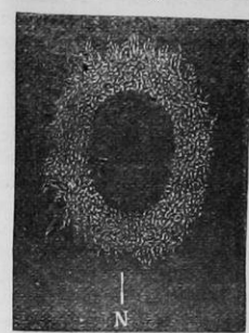
FIG. 4.—Ring nebula in Lyra, with its spectrum.
