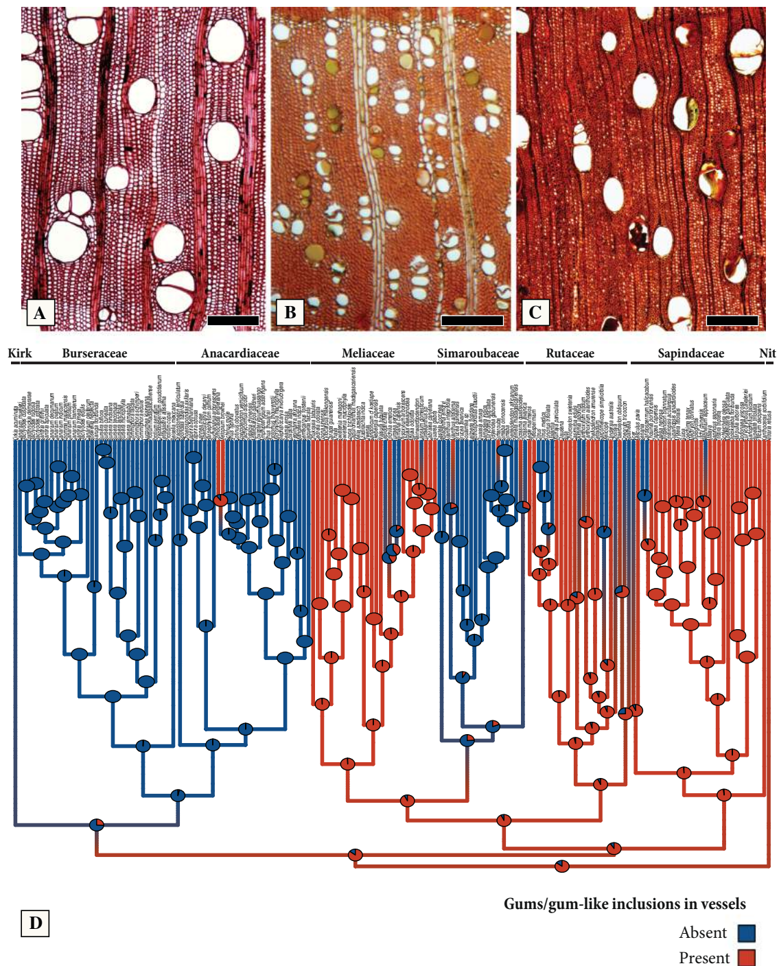
Fig. 7 Gums/gum-like deposits evolution in Sapindales. Transverse sections. a Spondias mombin L. (Anacardiaceae), gums/gum-like deposits absent. b Zanthoxylum caribaеum Lam. (Rutaceae), gums/gum-like deposits common. c Cupania macrophylla Mart. (Sapindaceae), gums/gum-like deposits common. d Ancestral character state estimation of gums/gum-like deposits present and their evolution in Sapindales. Scale bars: A, C = 300 \mu m; B = 150 \mu m. Kirk = Kirkiaceae, Nit = Nitrariaceae
