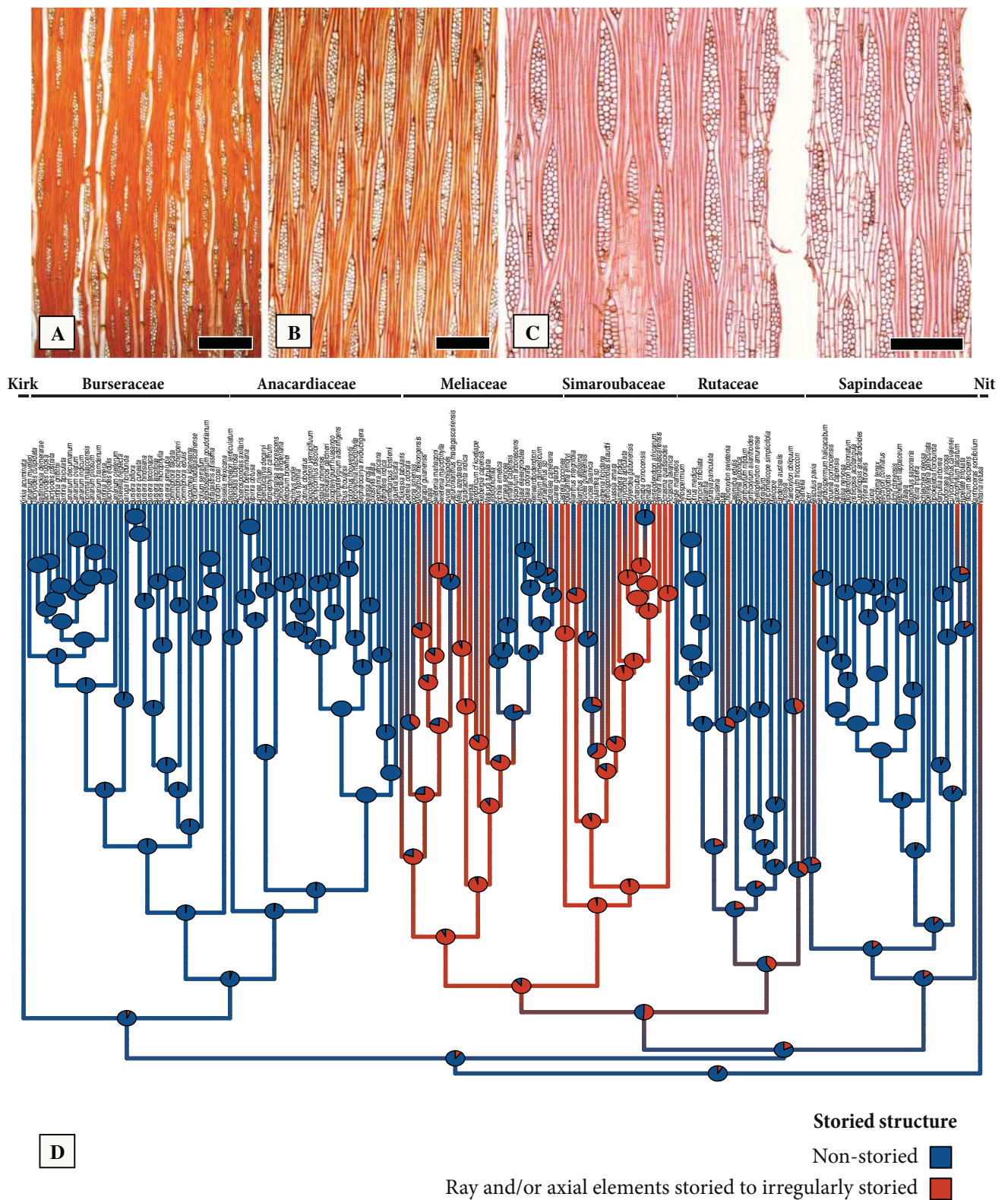
Fig. 15 Storied structure diversity and evolution in Sapindales. a-c. Longitudinal tangential sections. a Zanthoxylum caribaeum Lam. (Rutaceae), storied structure absent. b Swietenia macrophylla King. (Meliaceae), rays irregularly storied. c Simarouba glauca DC. (Simaroubaceae), rays and axial parenchyma storied. d Ancestral character state estimation of storied structure evolution. Scale bars: A-C = 300 \mu m. Kirk = Kirkiaceae, Nit = Nitrariaceae
