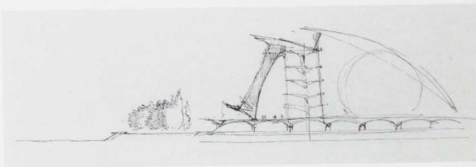
Science Museum. Preliminary sketch of section
