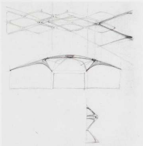
Preliminary sketches. Platform roof structure and cross section through platforms
