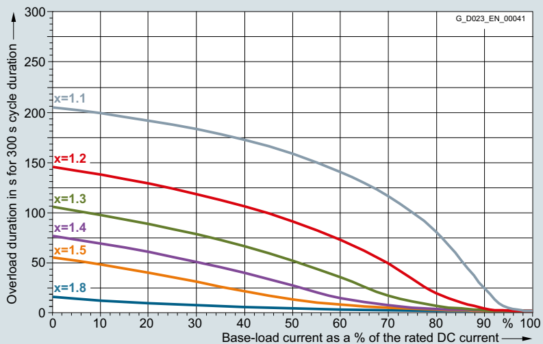
6RA8087-6DV62-0AA0 850 A/four-quadrant operation 400 V, 6RA8087-6FV62-0AA0 850 A/four-quadrant operation 480 V, 6RA8087-6GV62-0AA0 850 A/four-quadrant operation 575 V
