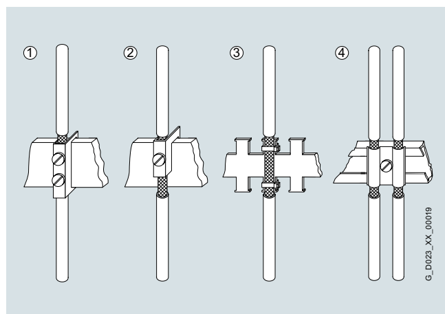
Shield connection
