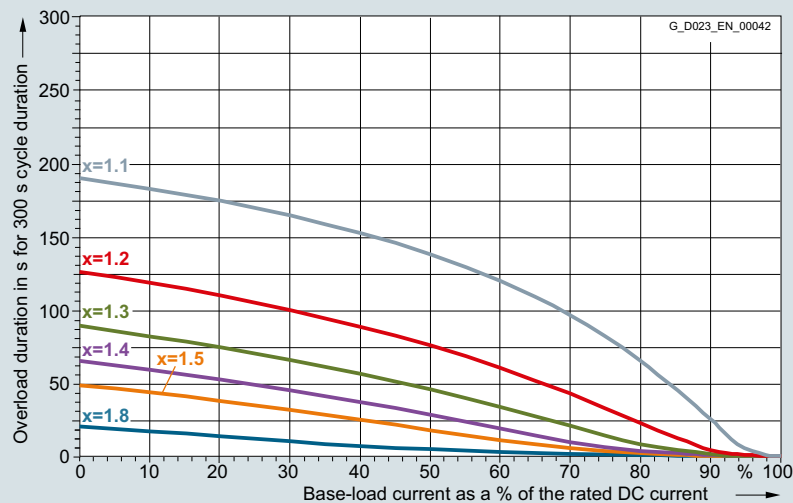
6RA8087-6GS22-0AA0 800 A/two-quadrant operation 575 V
