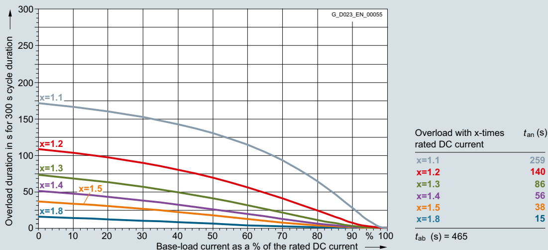
6RA8096-4MS22-0AA0 2200 A/two-quadrant operation 950 V, 6RA8096-4MV62-0AA0 2200 A/four-quadrant operation 950 V
