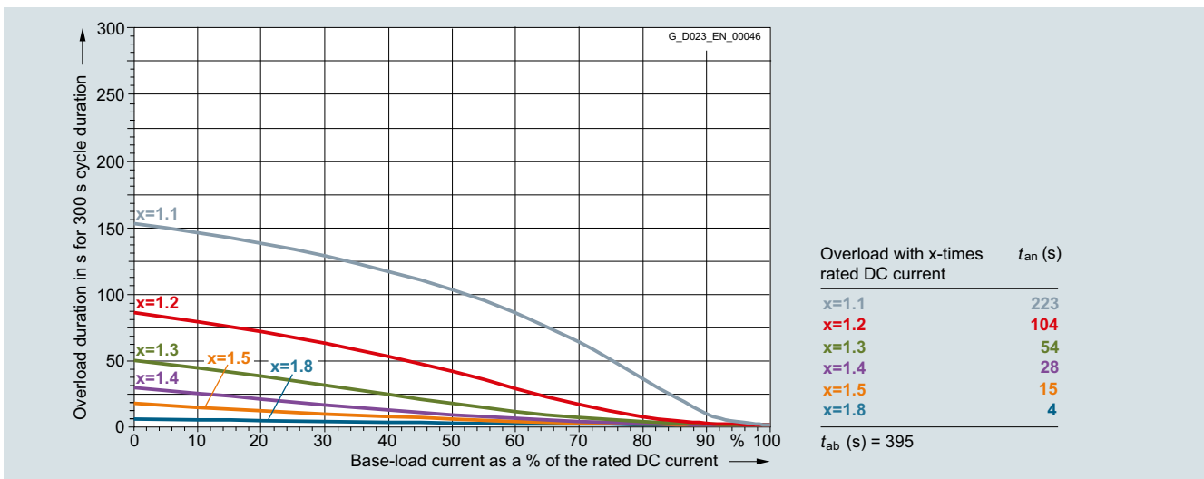
6RA8091-6DS22-0AA0 1200 A/two-quadrant operation 400 V, 6RA8091-6FS22-0AA0 1200 A/two-quadrant operation 480 V, 6RA8091-6FV62-0AA0 1200 A/four-quadrant operation 480 V, 6RA8091-6DV62-0AA0 1200 A/four-quadrant operation 400 V
