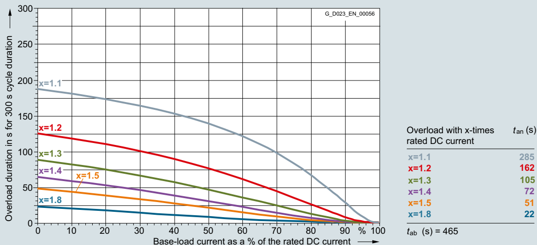
6RA8097-4GS22-0AA0 2800 A/two-quadrant operation 575 V, 6RA8097-4GV62-0AA0 2800 A/four-quadrant operation 575 V
