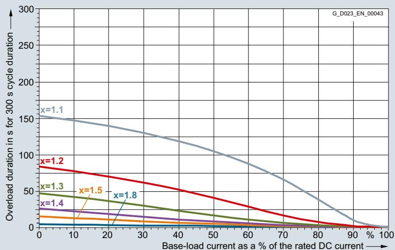
6RA8088-6LS22-0AA0 950 A/two-quadrant operation 830 V, 6RA8088-6LV62-0AA0 950 A/four-quadrant operation 830 V
