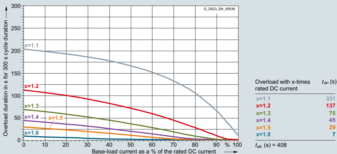
6RA8085-6DS22-0AA0 600 A/two-quadrant operation 400 V, 6RA8085-6FS22-0AA0 600 A/two-quadrant operation 480 V, 6RA8085-6GS22-0AA0 600 A/two-quadrant operation 575 V
