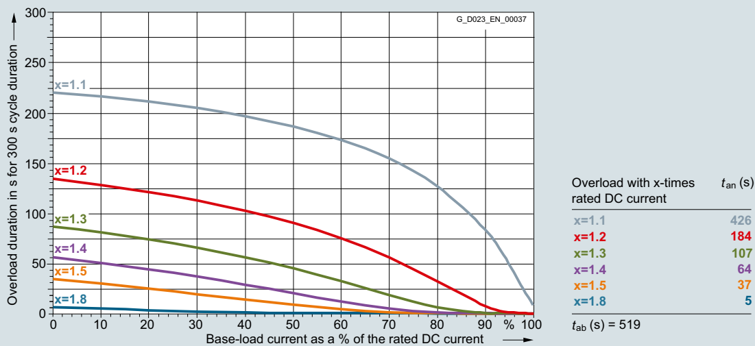
6RA8085-6DV62-0AA0 600 A/four-quadrant operation 400 V, 6RA8085-6FV62-0AA0 600 A/four-quadrant operation 480 V, 6RA8085-6GV62-0AA0 600 A/four-quadrant operation 575 V
