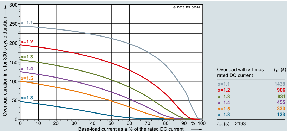
6RA8018-6DV62-0AA0 30 A/four-quadrant operation 400 V, 6RA8018-6FV62-0AA0 30 A/four-quadrant operation 480 V
