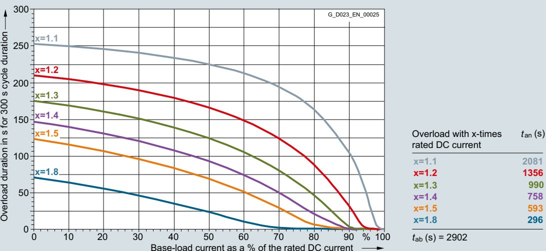
6RA8025-6DS22-0AA0 60 A/two-quadrant operation 400 V, 6RA8025-6FS22-0AA0 60 A/two-quadrant operation 480 V, 6RA8025-6GS22-0AA0 60 A/two-quadrant operation 575 V
