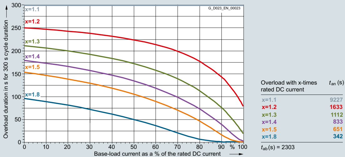
6RA8013-6DV62-0AA0 15 A/four-quadrant operation 400 V, 6RA8013-6FV62-0AA0 15 A/four-quadrant operation 480 V
