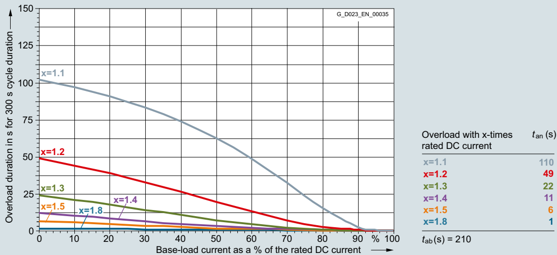
6RA8082-6FS22-0AA0 450 A/two-quadrant operation 480 V, 6RA8082-6FV62-0AA0 450 A/four-quadrant operation 480 V
