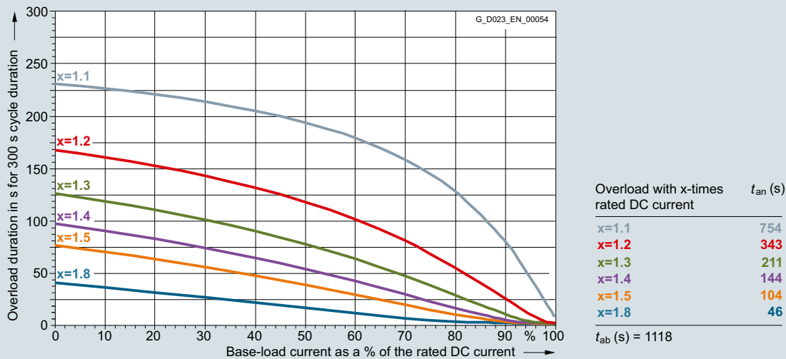
6RA8096-4GS22-0AA0 2200 A/two-quadrant operation 575 V, 6RA8096-4GV62-0AA0 2200 A/four-quadrant operation 575 V
