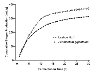
Cumulative biogas production
