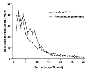
Daily biogas production
