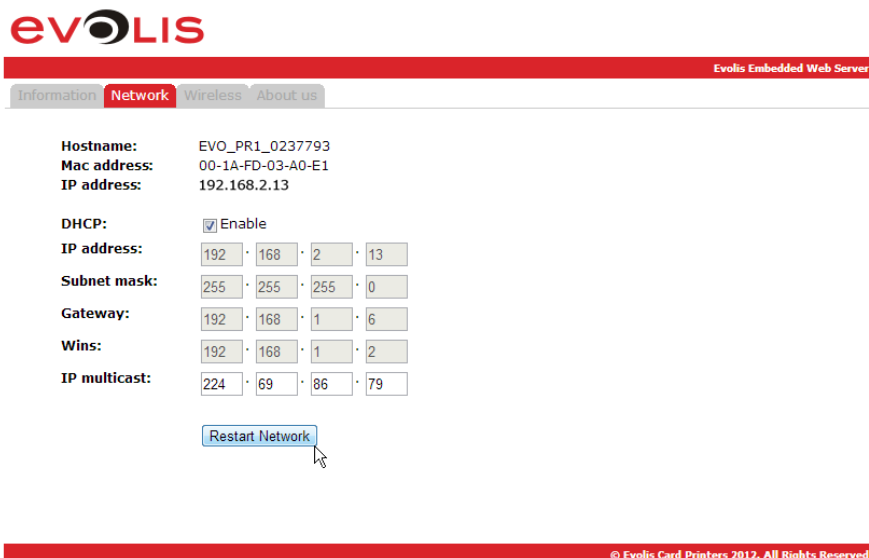
Figure 9: Web server (DHCP mode)
