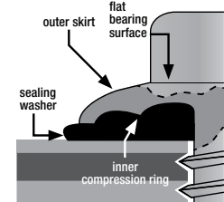
Drill Screw with Flo-Seal System
