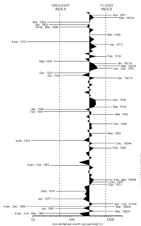
Fig. 8. Extreme rainfall months at Hilo airport from 1900 to 1984. Months with <50 mm (2 in.) rain are shown left of drought index and those with >750 mm (30 in.) at right of flood index. Months marked with an asterisk (*) indicate intense drought or flood events (reproduced with permission from Annual Review of Ecology and Systematics, 17, 231, 1986).
