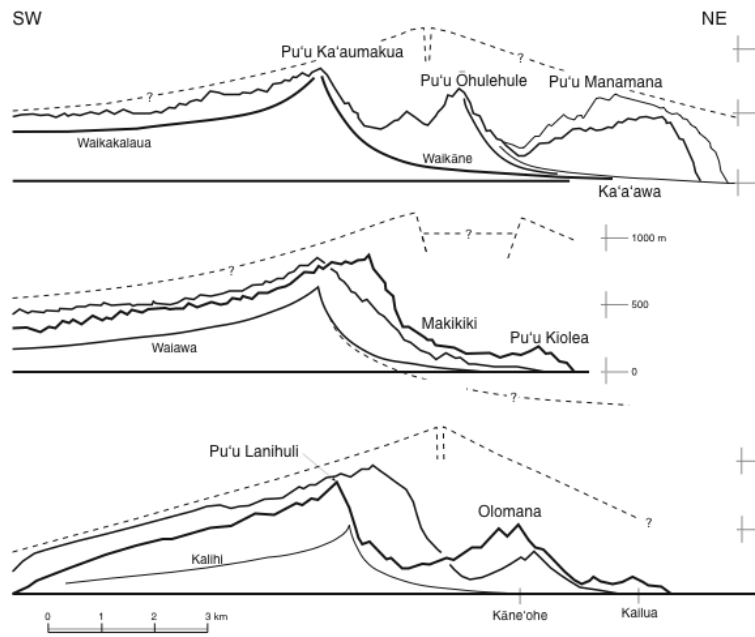
Fig. 15. This diagram (from Wirthmann and Hueser, 1987) demonstrates the outcome of breakdown of a Hawaiian shield volcano. The diagram shows three topographic profiles crossing from SW to NE through the windward Ko'olau mountain range of O'ahu Island. The slope reduction to this level of contemporary topography took 2.6 million years on the rain- and trade wind exposed west side of the island. In addition to regular stream erosion there were sudden break-offs of whole slope segments that rolled into the ocean, where they now form small, offshore islands.
