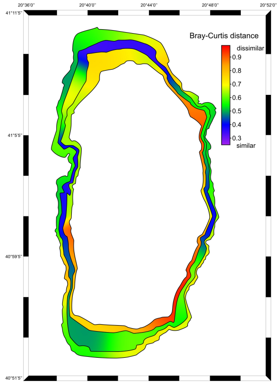
Fig. 6. Similarity map of the thanatocoenosis of core Co1200 and recent gastropod communities in ancient Lake Ohrid. Three zones are shown: Surface Layer (0–5 m), Intermediate Layer (5–25 m), and Deep Layer (25–50 m). Note that the extents of the zones are not to scale with Albrecht and Wilke (2008).
