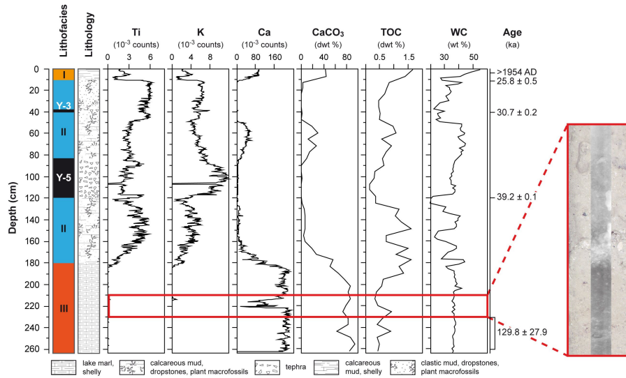
Fig. 2. Lithofacies, lithology, Ti-, K-, Ca-intensities, CaCO 3 , total organic carbon (TOC) dry weight percentages, water content (WC), and age control points of core Co1200. The red framed optical and radiographic images to the right show a horizon at 220 cm which consisted almost entirely of intact and broken mollusc fossils.
