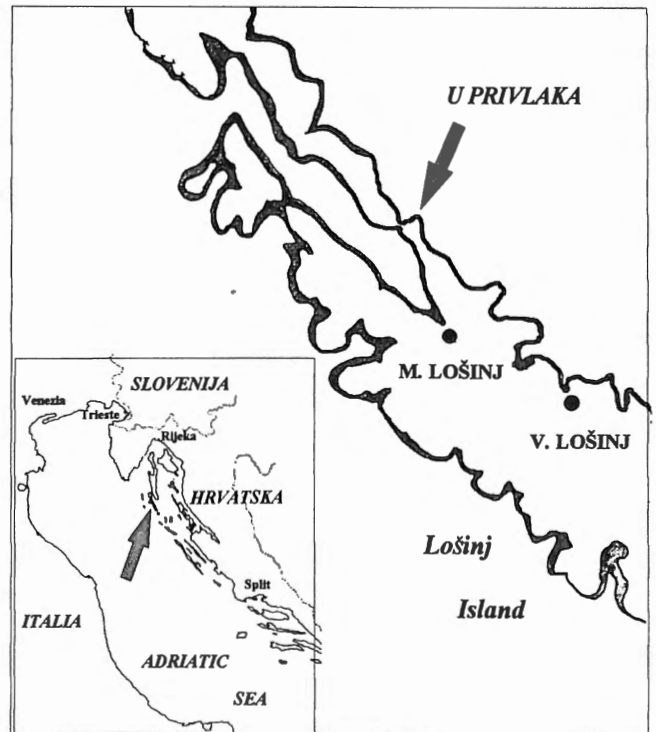
Fig. 1. – Map illustrating the area of Lošinj Island (northern Adriatic, Croatia) and a detail of Lošinj Island with situation of the submarine cave at U Privlaka.
