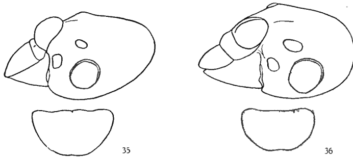
FIG. 35-36. — Ancistrotermes . Head in lateral view, and pronata of imagoes : 35, A. latinotus ; 36, A. crucifer .
