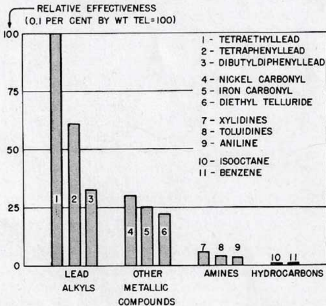
Figure 1. Relative Effectiveness of Antiknock Compounds
