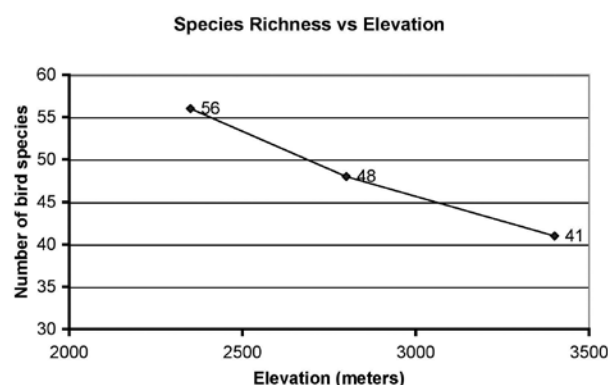
Figure 3.1. Elevational trend in species richness of birds in the Kaijende Highlands.
