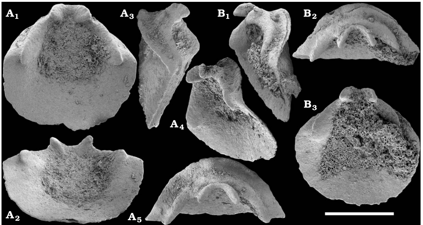
Fig. 31. Hyolith opercula Parkula cf. P. esmeraldina Skovsted, 2006 from lower Cambrian Emyaksin Formation, Malaya Kuonamka River, Anabar Uplift, Siberia; sample K1-3B. A. SMNH X 4660; inner (A 1 ), oblique ventral (A 2 ), lateral (A 3 , A 4 ), and dorsal (A 5 ) views. B. SMNH X 4661; lateral (B 1 ), dorsal (B 2 ), and inner (B 3 ) views. Scale bar 300 \mu m.
