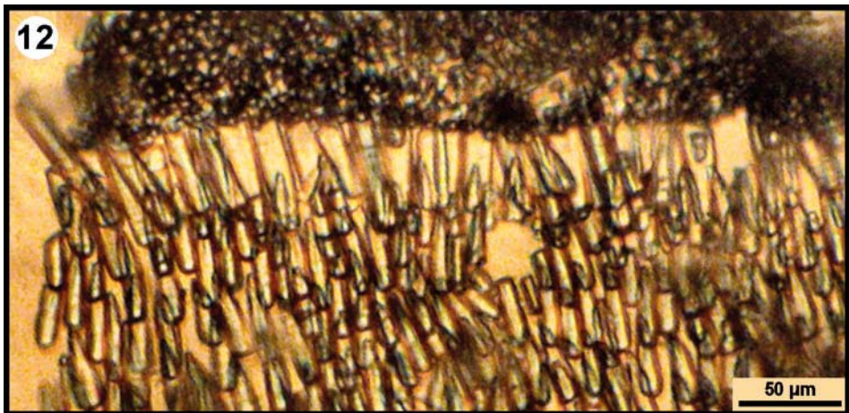
Fig. 12. Lepidochitona (L.) dicksaе , holotype V6152/T1539: spicules of girdle with edge of perinotum.
