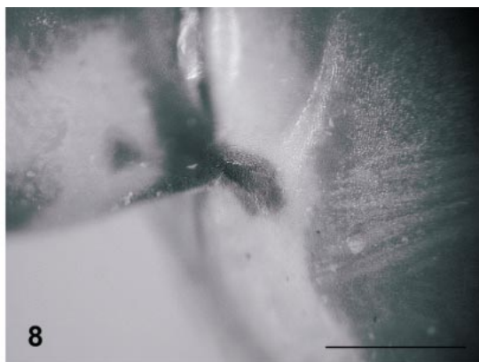
Figs. 7–8. Thyridium on second metasomal tergum of female. 7, Asteloeca traili (Cameron); 8, Asteloeca ujhelyii (Ducke). All scale bars are 0.5 mm.
