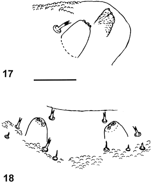
Figs. 17–18. Final instar larva of Asteloeca ujhelyii . 17, apical part of maxilla; 18, labial palpi and area around them. The scale bar is 0.1 mm.
