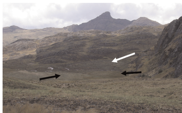
FIGURE 2. View of wetland Cocañes 3 looking southeast, illustrating its three major groundwater flow systems indicated by arrows. The water flowing from the near side of the wetland (two black arrows) has pH ranging from 6.4 to 6.7, while that from the far side (white arrow) is highly acid with pH ranging from 4.3 to 4.7. The two areas support different plant species and plant communities.
