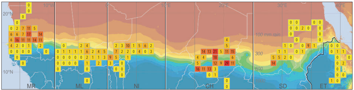
Figure S3. Woody cover (%) of Balanites aegyptiaca ; present in 72% of the 150 cells. Average woody cover (mean \pm SD) in grid cells: 3.5% \pm 5.4.
