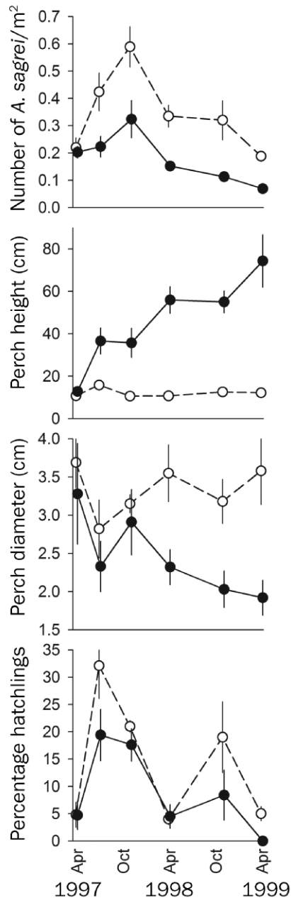
Figure 11. Effect of introduction of predatory lizards ( Leiocephalus carinatus ) on Anolis sagrei populations, in terms of (a) population density, (b) perch height, (c) perch diameter, and (d) percentage of lizards observed that were hatchlings. Modified from Schoener and colleagues (2002).
