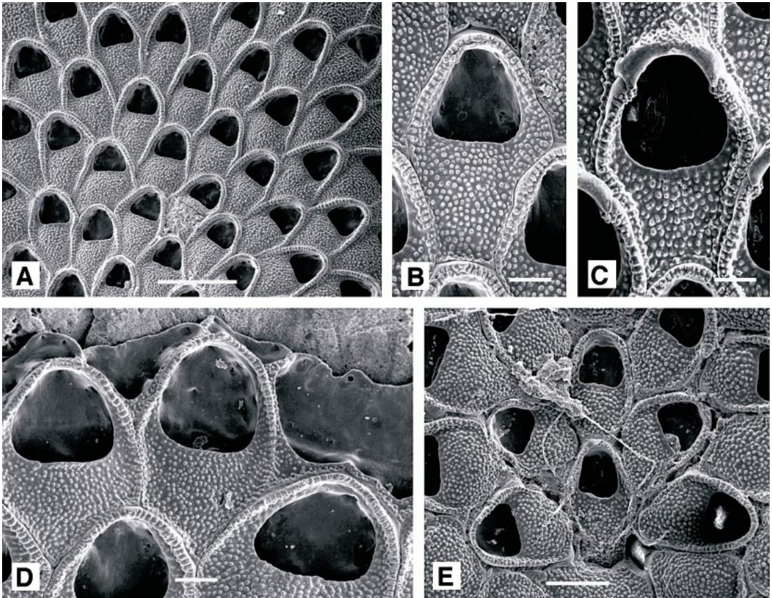
Fig. 14. A–E. Rosseliana rosselii . A. General aspect (AMNH 1053; 0.5 mm). B. Autozooid (AMNH 1053; 0.1 mm). C. Maternal zoid with largely immersed ovicell (AMNH 1054; 0.1 mm). D. Growing edge of colony (AMNH 1055; 0.10 mm). E. Ancestrula and early autozooids (AMNH 1055; 0.2 mm).
