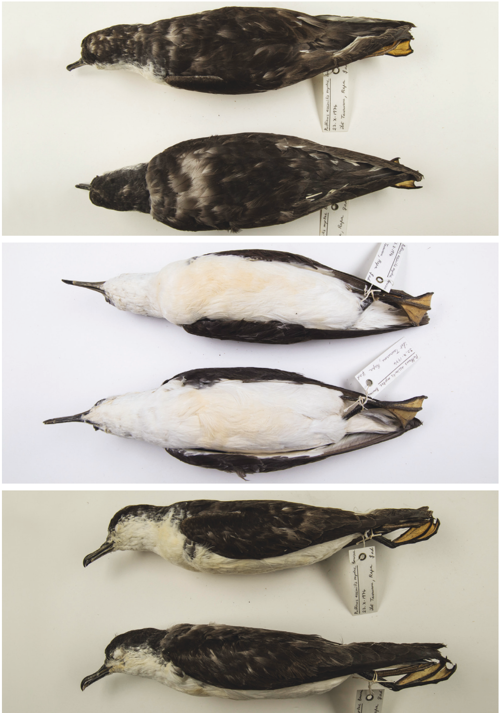
Figure 2. Dorsal, ventral and lateral views of two adult female Rapa Shearwaters, taxon myrtae (MNHN 1789.1975, below, and MNHN 1787.1975), collected on Tauturuu, off Rapa Island, Polynesia, October 1974; unlike the holotype (a juvenile), note especially the much darker and more uniform upperparts (Hadoram Shirihai, Tubenoses Project / © Muséum National d'Histoire Naturelle, Paris)
