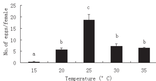
Fig. 1. Egg production by Conopomorpha sinensis females at different temperatures. Different lower case letters above bars show significantly different results at P < 0.05 (Tukey's test).
