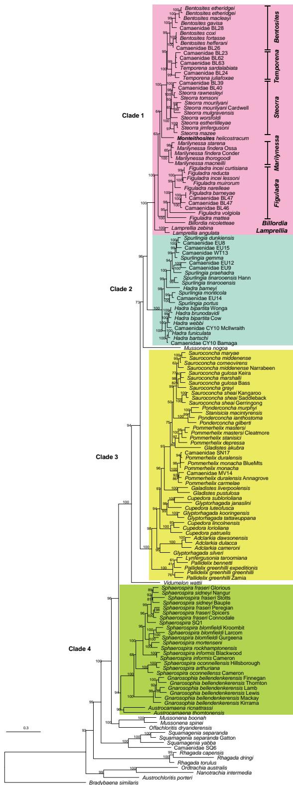
Fig. 1. Maximum Likelihood tree based on analysis of GenBank sequences representing the clades I to 4 in the tree depicted by Hugall and Stanisic (2011, fig. 7) showing a reconstruction of the phylogenetic relationships among the Eastern Australian hadroid snails. Species names have been updated in accordance with the current taxonomy proposed by Stanisic et al. (2010). Phylogeny courtesy of Andrew Hugall.
