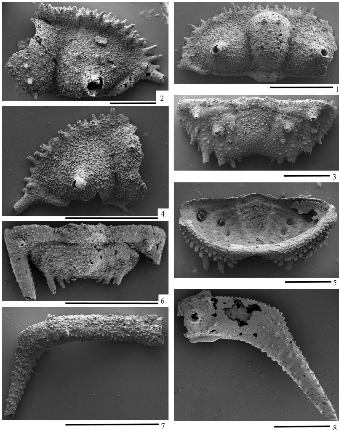
Figure 4. (1–8) Cyphaspidetes ammari new species. (1–5, 7) From the mined trilobite bed at Talawarite locality (Fig. 1), of early Eifelian age, belonging to the Bou Tchrafine Formation, close to the top of the mountain. (6, 8) From the trilobite beds where phacopid trilobites that are red in color are sometimes preserved with greenish eye lenses at Hamar Laghdad (Red-Green Hamar Laghdad locality in Fig. 1), of Eifelian age, also from the Bou Tchrafine Formation. (1) Dorsal view of incomplete cephalon, paratype UA14318. (2) Dorsal view of fragment of cephalon, paratype UA14319. (3) Dorsal view of small pygidium, paratype UA14320. (4) Dorsal view of fragment of cephalon, paratype UA14321. (5) Ventral view of small pygidium, paratype UA14322. (6) Dorsal view of transitory pygidium, plesiotype UA14323. (7) Dorsal view of fragment (left pleura) of small thoracic segment, paratype UA14324. (8) Dorsal view of fragment (right pleura) of thoracic segment, plesiotype UA14268. Scale bars = 1 mm.
