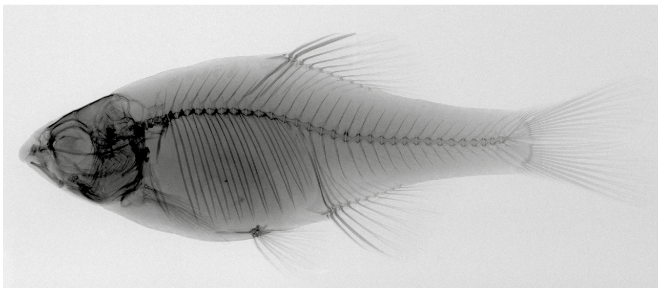
Fig. 3. Radiograph of Rhodeus cyanorostris sp. nov. (SOU 1801002, paratype, ♂, 33.2 mm SL).
