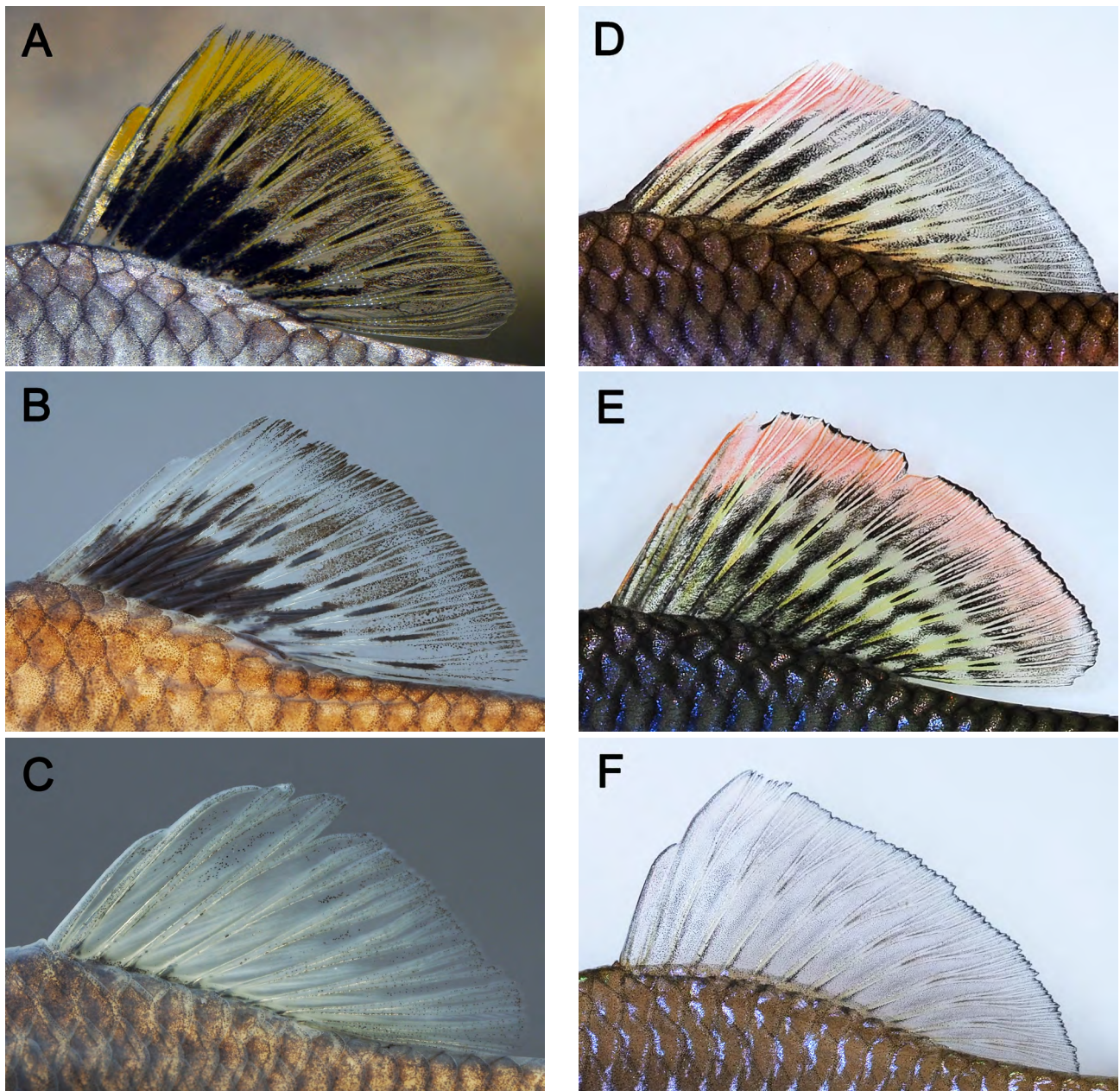
Fig. 15. Dorsal fin of adult males of five Rhodeus species. A) R. nigrodorsalis sp. nov. in life, SOU 1903001, 47.1 mm SL; B) R. nigrodorsalis sp. nov. in preservative, SOU 1712002, 37.9 mm SL; C) R. cyanostris sp. nov. in preservative, SOU 1801001, holotype, 32.1 mm SL; D) R. amarus in life, 59.8 mm SL (specimen not preserved), collected from Ballica, Turkey; E) R. shitaiensis in life, 56.1 mm SL (specimen not preserved), collected from Shitai County, Anhui Province, China; F) R. rheinardti in life, 49.3 mm SL (specimen not preserved), collected from Hue City, Vietnam.
