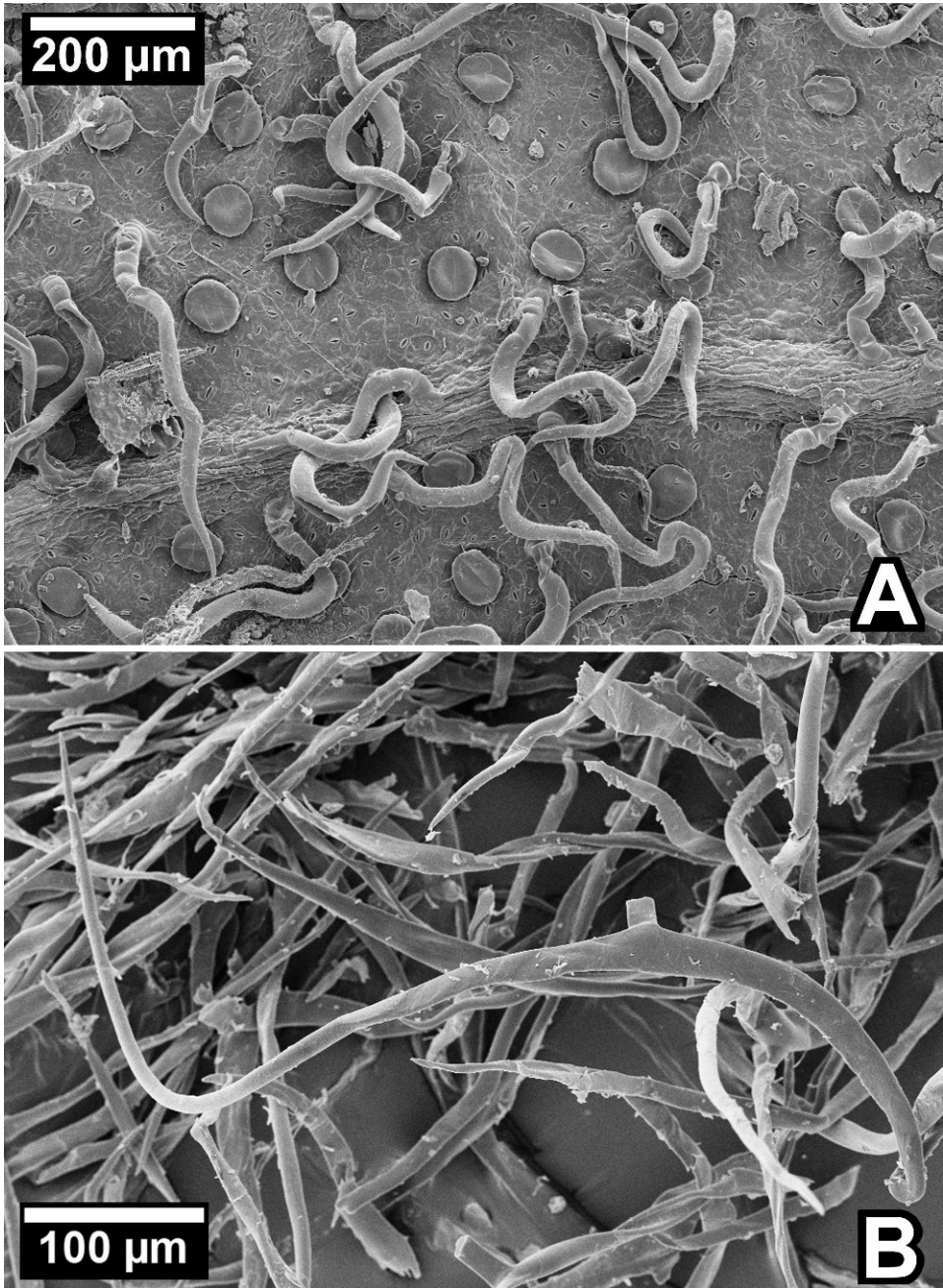
Fig. 3. SEM of trichomes from abaxial surfaces of leaf blades. A, Strobocalyx arborea showing simple hairs (Tonkin, Pételot 6624, US); B, Tarlounia elliptica showing short-stalked T-shaped hairs (Sri Lanka, Grierson 1013, US).
