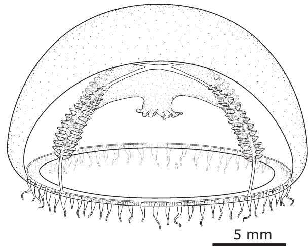
Fig. 5. Ptychogena lactea , subadult, schematic after MHNG-INVE-82311.
