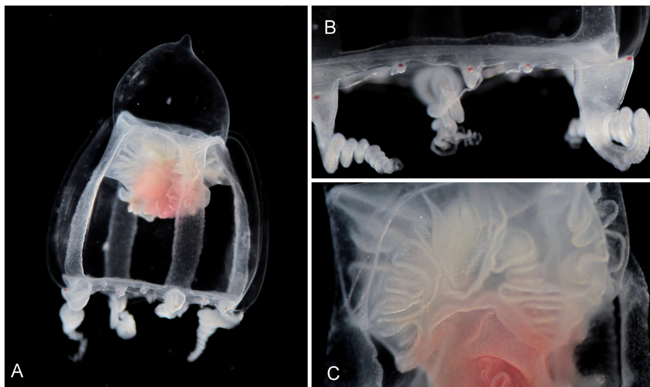
Fig. 17. Leuckartiara spec., living animal. (A) Whole medusa. (B) Bell margin with tentacle bases. (C) Details of manubrium with gonad folds (immature?).
