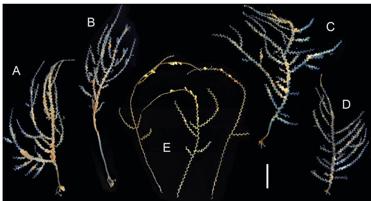
Fig. 3. Sertularella malagasiensis sp. nov. Four colonies (A-D) compared to three colonies of S. polyzonias (Linnaeus, 1958) (E), to show differences. Scale bar: 1 cm (A-E).
